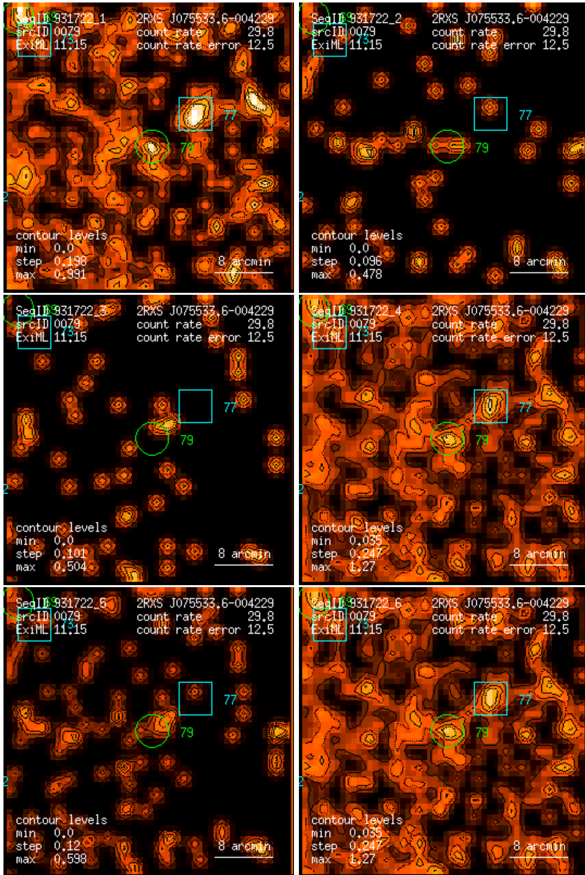
Figure 79: RASS 931722: detection 0079: band rate images, Gaussian filter: (1) PSPC channels 11 – 41, (2) 52 – 90, (3) 91 – 201, (4) 11 – 235, (5) 52 – 201, (6) 11 – 201. Broad band rates in counts/ks. Band rate contour levels in counts/ks/arcmin 2 .
