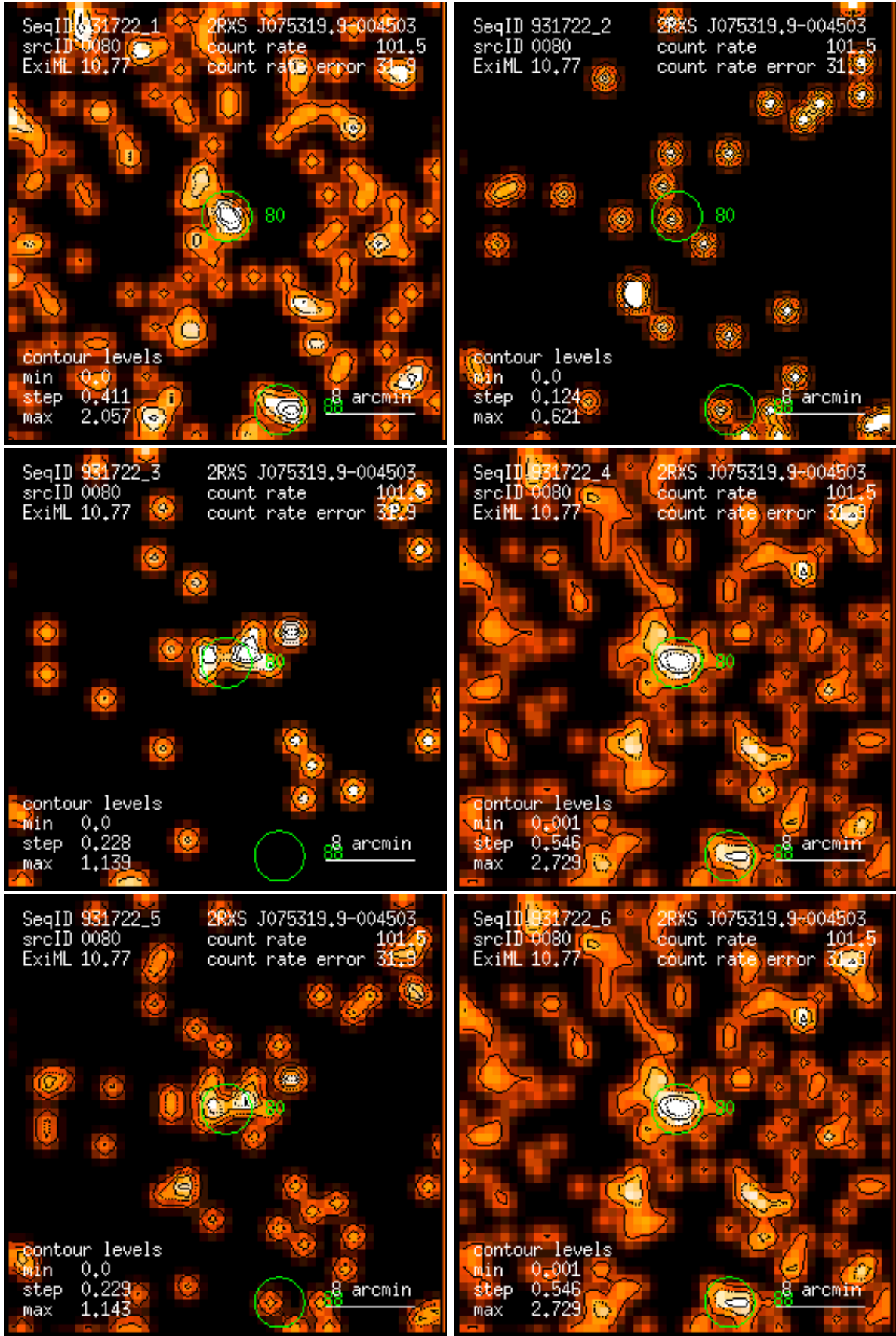
Figure 80: RASS 931722: detection 0080: band rate images, Gaussian filter: (1) PSPC channels 11 – 41, (2) 52 – 90, (3) 91 – 201, (4) 11 – 235, (5) 52 – 201, (6) 11 – 201. Broad band rates in counts/ks. Band rate contour levels in counts/ks/arcmin 2 .
