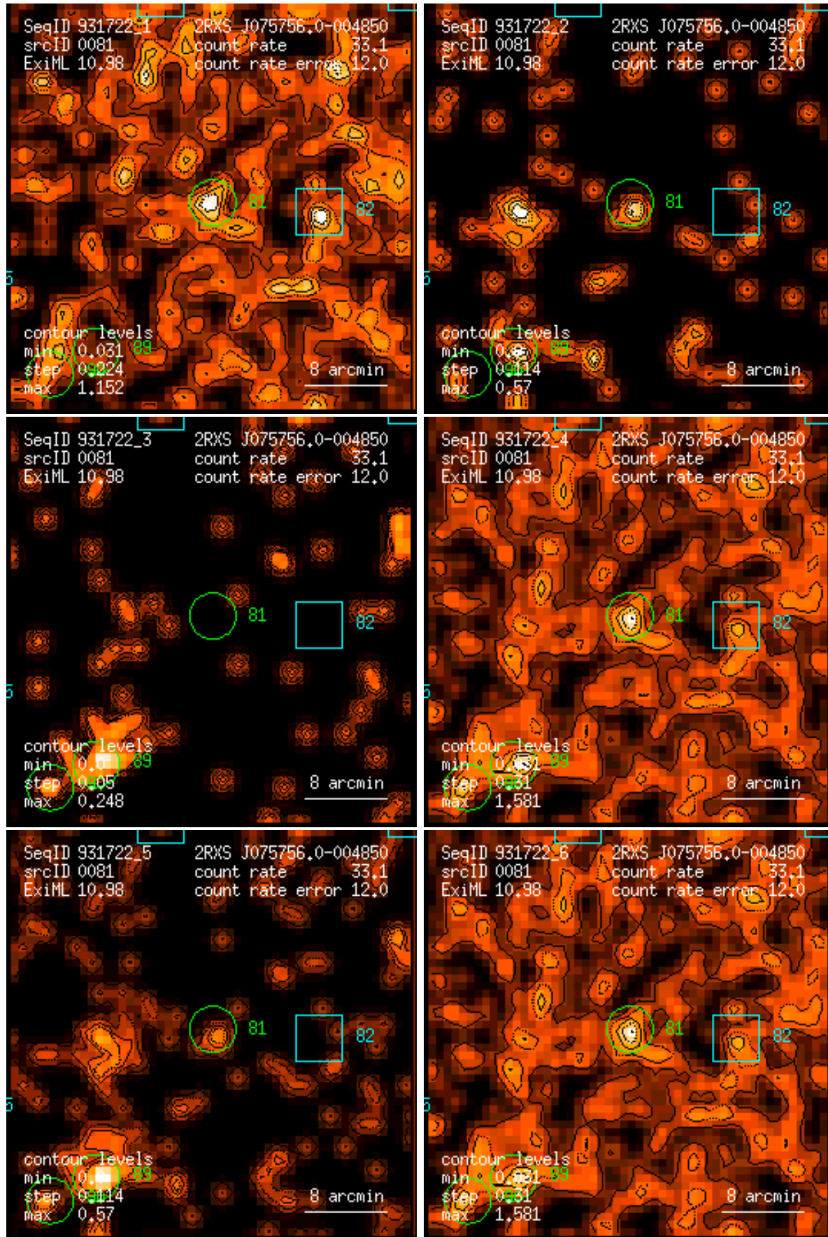
Figure 81: RASS 931722: detection 0081: band rate images, Gaussian filter: (1) PSPC channels 11 – 41, (2) 52 – 90, (3) 91 – 201, (4) 11 – 235, (5) 52 – 201, (6) 11 – 201. Broad band rates in counts/ks. Band rate contour levels in counts/ks/arcmin 2 .
