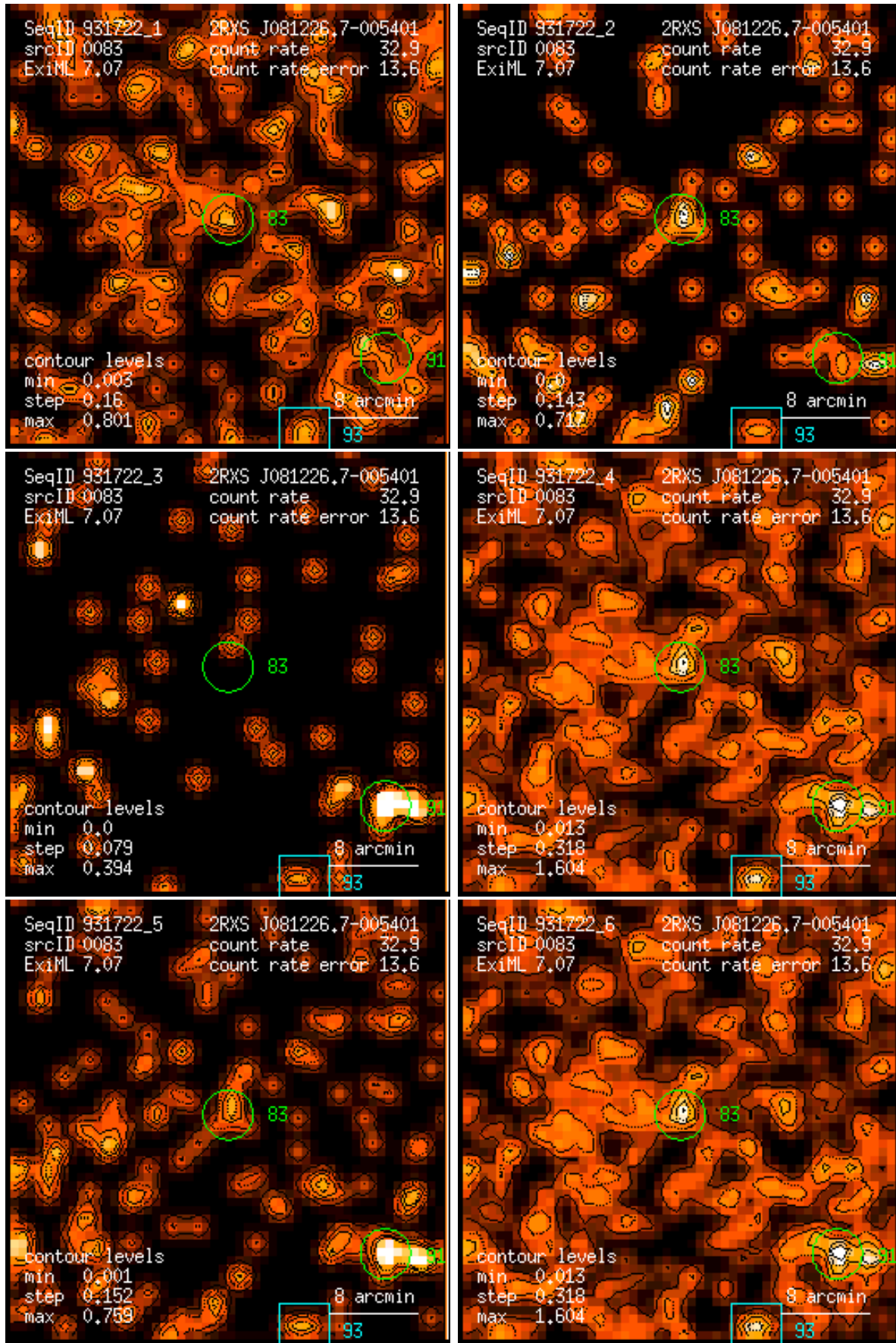
Figure 83: RASS 931722: detection 0083: band rate images, Gaussian filter: (1) PSPC channels 11 – 41, (2) 52 – 90, (3) 91 – 201, (4) 11 – 235, (5) 52 – 201, (6) 11 – 201. Broad band rates in counts/ks. Band rate contour levels in counts/ks/arcmin 2 .
