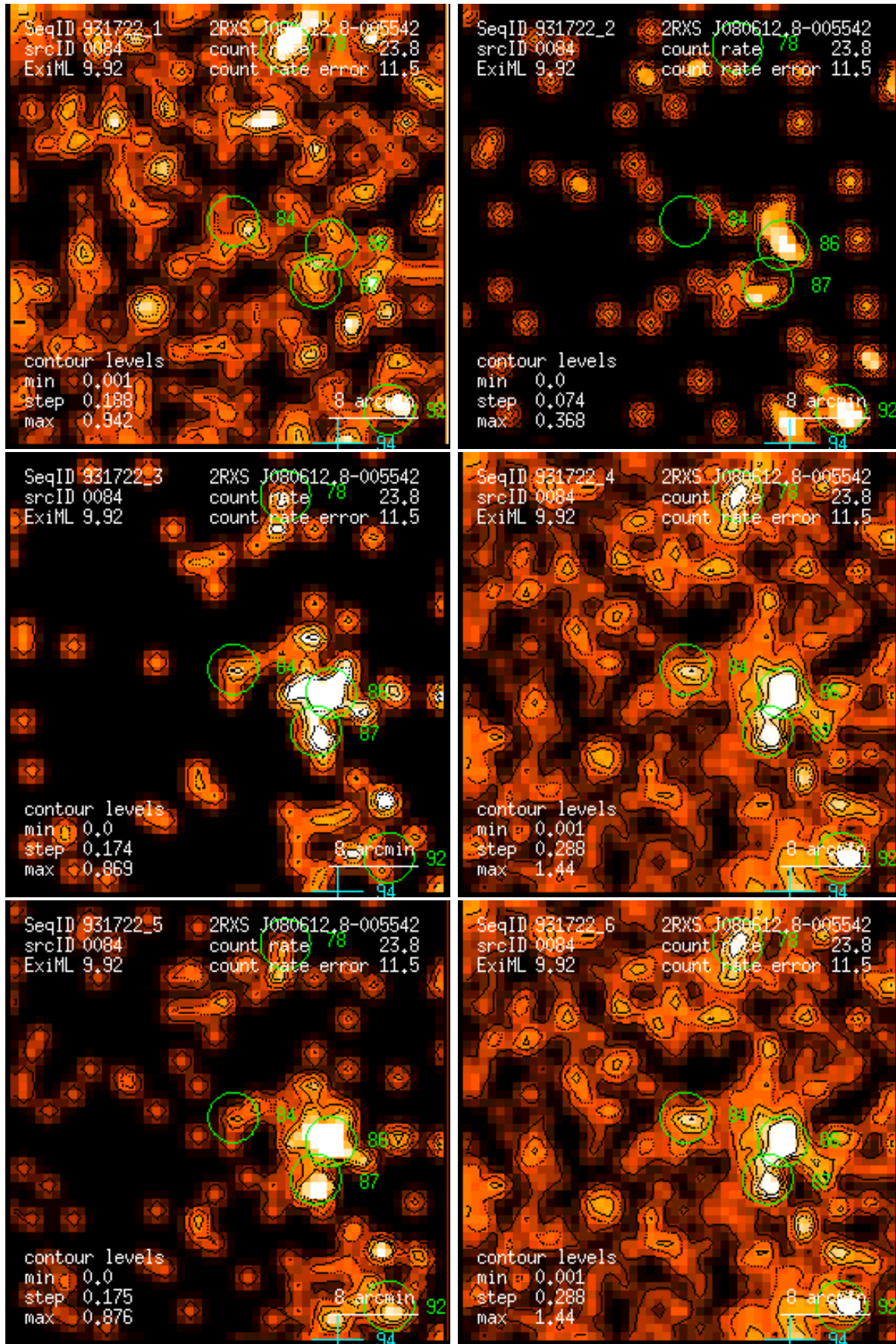
Figure 84: RASS 931722: detection 0084: band rate images, Gaussian filter: (1) PSPC channels 11 – 41, (2) 52 – 90, (3) 91 – 201, (4) 11 – 235, (5) 52 – 201, (6) 11 – 201. Broad band rates in counts/ks. Band rate contour levels in counts/ks/arcmin 2 .
