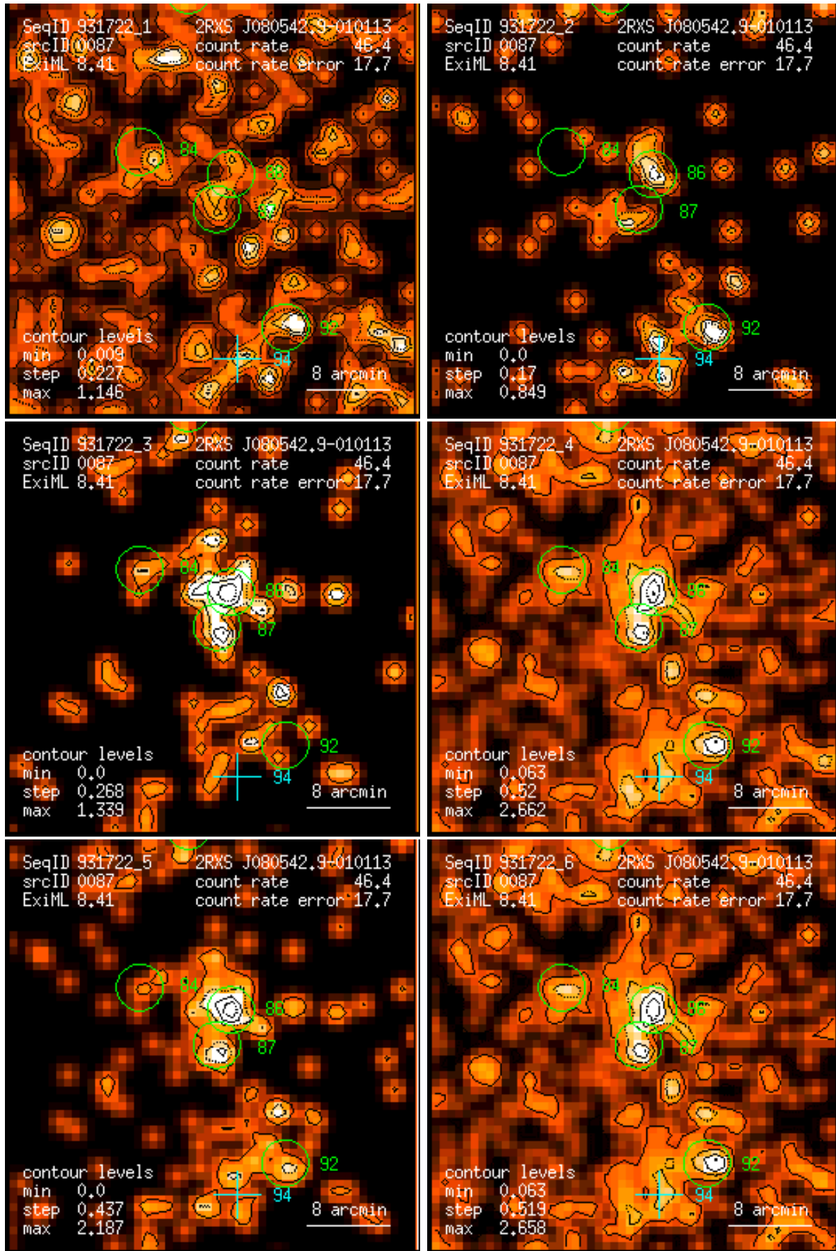
Figure 87: RASS 931722: detection 0087: band rate images, Gaussian filter: (1) PSPC channels 11 – 41, (2) 52 – 90, (3) 91 – 201, (4) 11 – 235, (5) 52 – 201, (6) 11 – 201. Broad band rates in counts/ks. Band rate contour levels in counts/ks/arcmin 2 .
