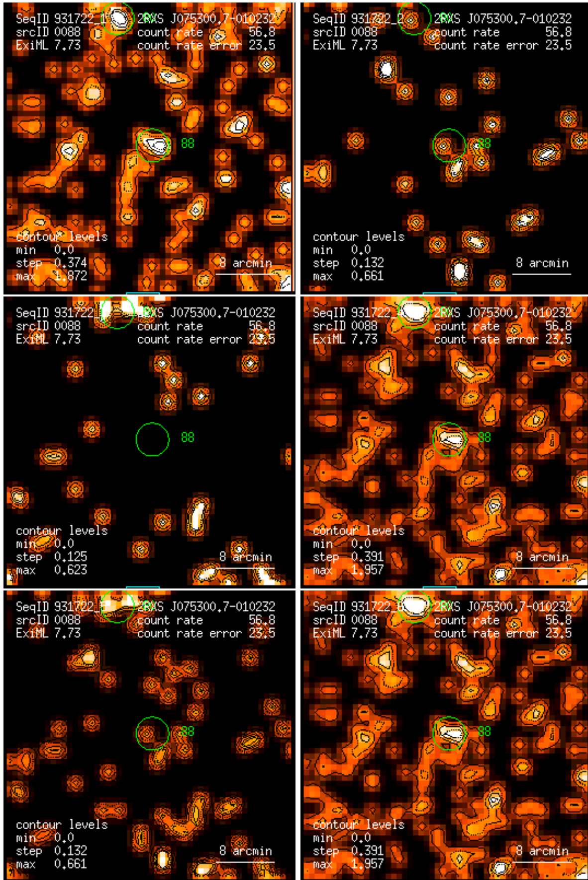
Figure 88: RASS 931722: detection 0088: band rate images, Gaussian filter: (1) PSPC channels 11 – 41, (2) 52 – 90, (3) 91 – 201, (4) 11 – 235, (5) 52 – 201, (6) 11 – 201. Broad band rates in counts/ks. Band rate contour levels in counts/ks/arcmin 2 .
