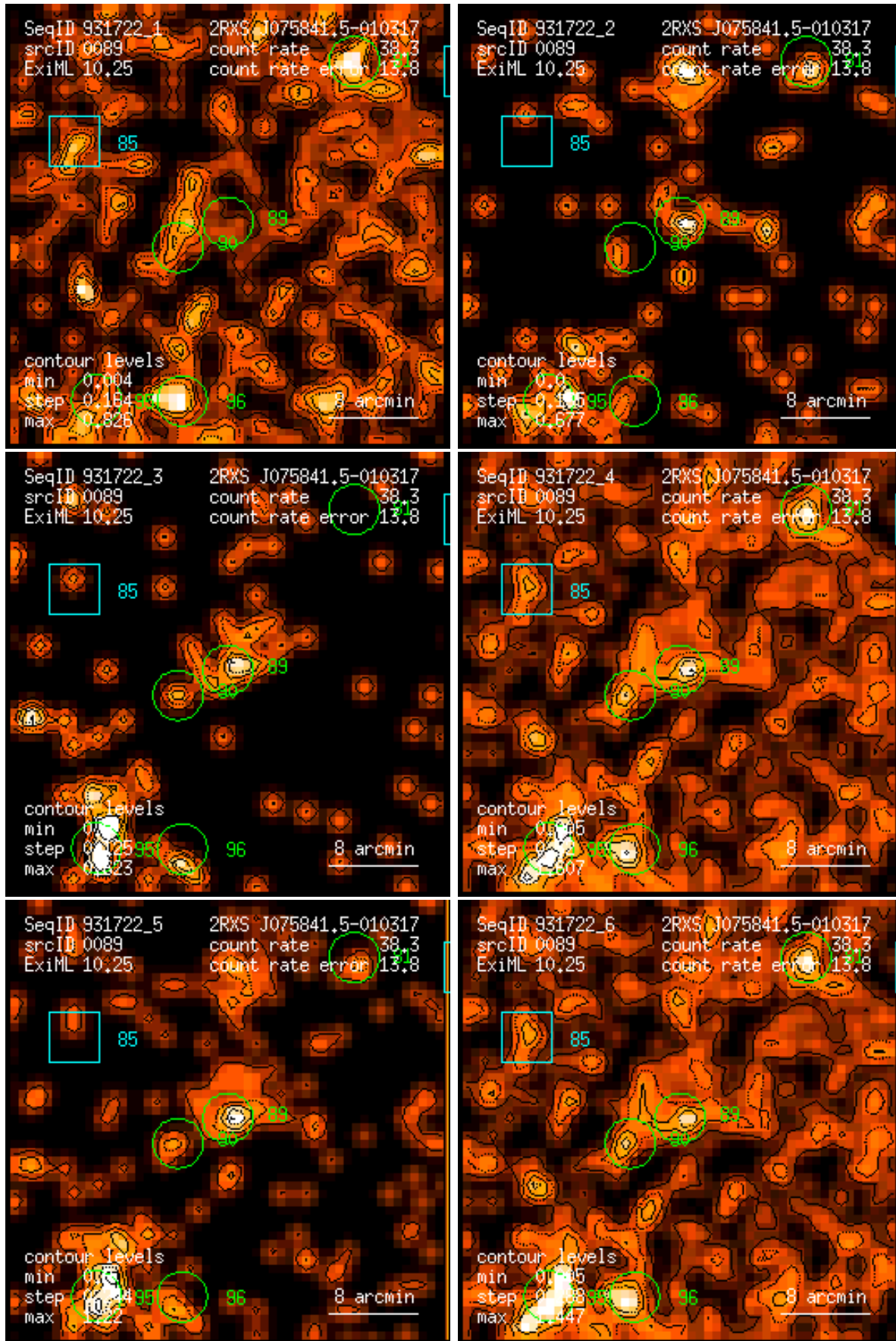
Figure 89: RASS 931722: detection 0089: band rate images, Gaussian filter: (1) PSPC channels 11 – 41, (2) 52 – 90, (3) 91 – 201, (4) 11 – 235, (5) 52 – 201, (6) 11 – 201. Broad band rates in counts/ks. Band rate contour levels in counts/ks/arcmin 2 .
