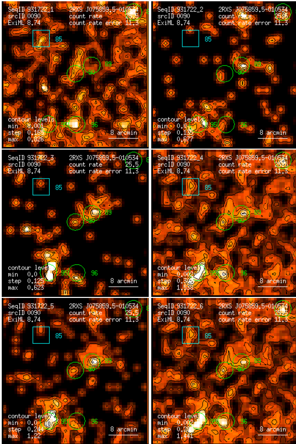
Figure 90: RASS 931722: detection 0090: band rate images, Gaussian filter: (1) PSPC channels 11 – 41, (2) 52 – 90, (3) 91 – 201, (4) 11 – 235, (5) 52 – 201, (6) 11 – 201. Broad band rates in counts/ks. Band rate contour levels in counts/ks/arcmin 2 .
