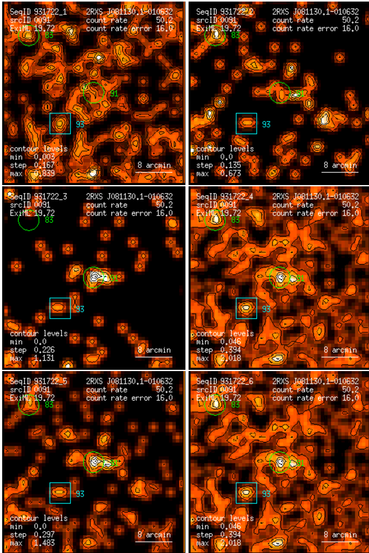
Figure 91: RASS 931722: detection 0091: band rate images, Gaussian filter: (1) PSPC channels 11 – 41, (2) 52 – 90, (3) 91 – 201, (4) 11 – 235, (5) 52 – 201, (6) 11 – 201. Broad band rates in counts/ks. Band rate contour levels in counts/ks/arcmin 2 .
