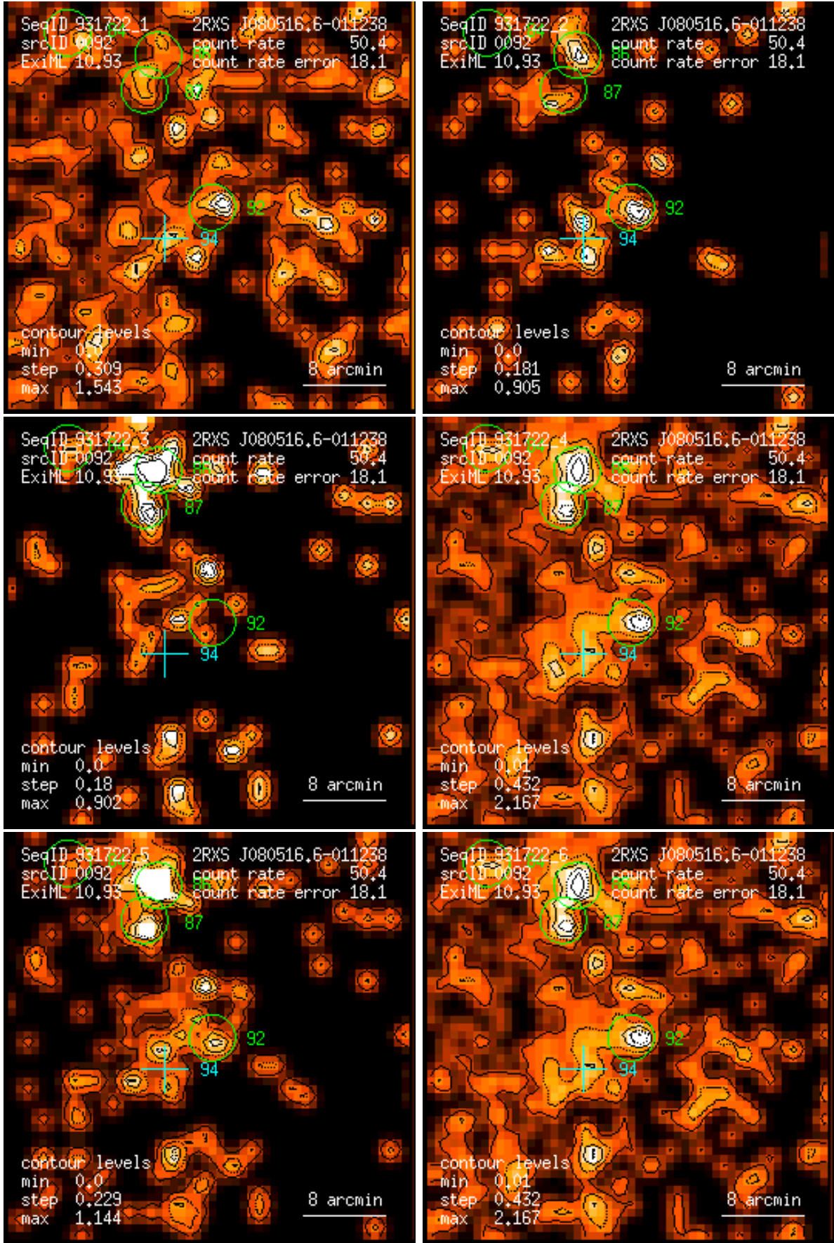
Figure 92: RASS 931722: detection 0092: band rate images, Gaussian filter: (1) PSPC channels 11 – 41, (2) 52 – 90, (3) 91 – 201, (4) 11 – 235, (5) 52 – 201, (6) 11 – 201. Broad band rates in counts/ks. Band rate contour levels in counts/ks/arcmin 2 .
