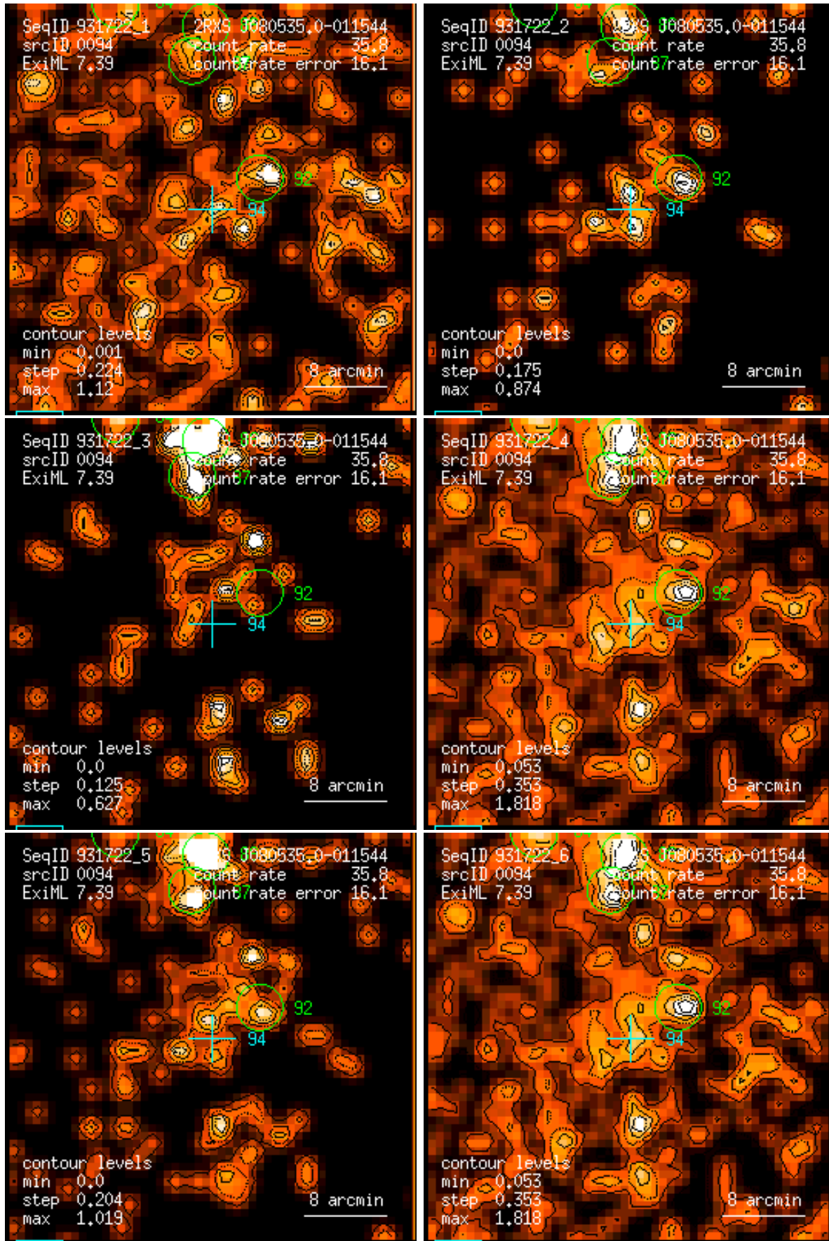
Figure 94: RASS 931722: detection 0094: band rate images, Gaussian filter: (1) PSPC channels 11 – 41, (2) 52 – 90, (3) 91 – 201, (4) 11 – 235, (5) 52 – 201, (6) 11 – 201. Broad band rates in counts/ks. Band rate contour levels in counts/ks/arcmin 2 .
