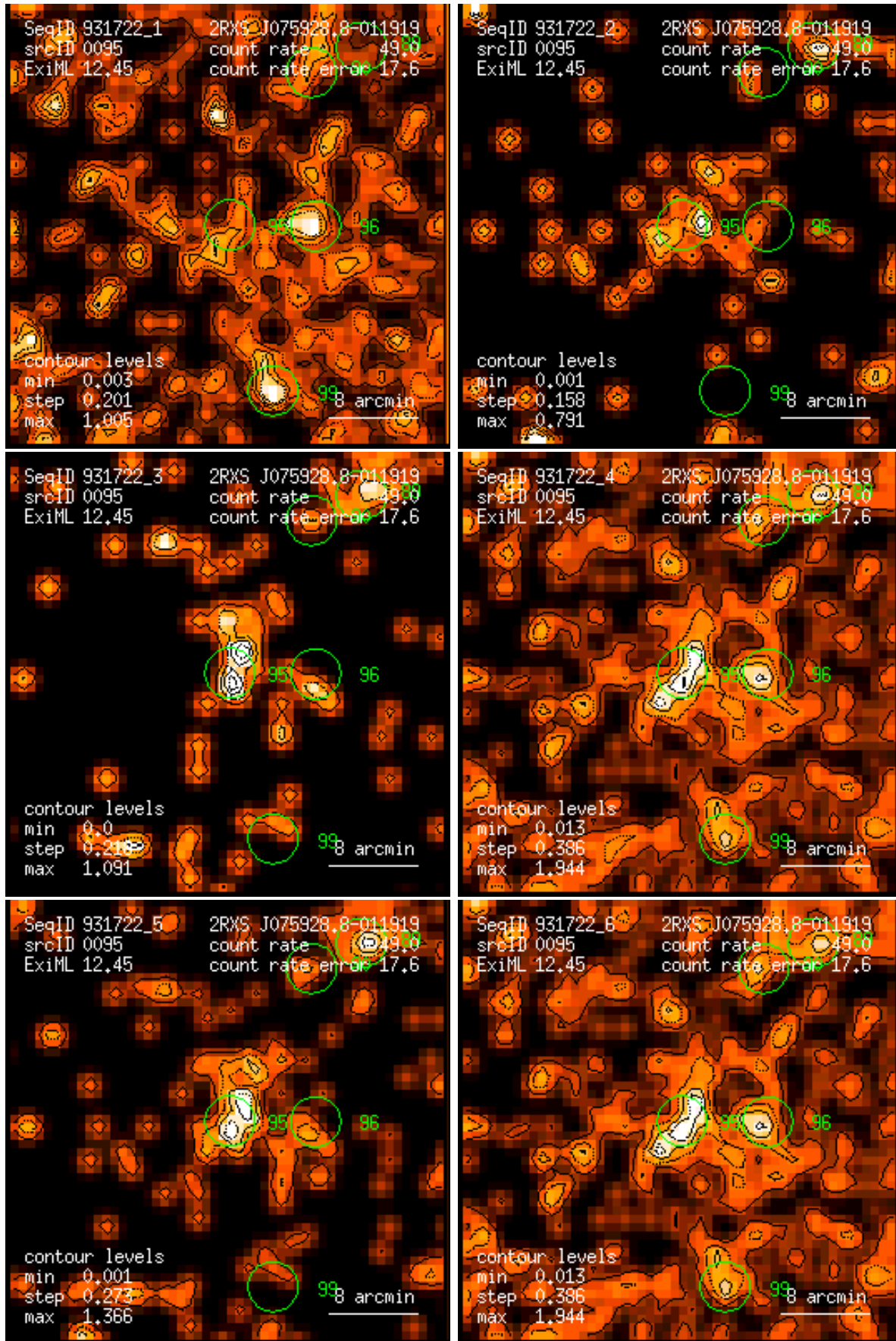
Figure 95: RASS 931722: detection 0095: band rate images, Gaussian filter: (1) PSPC channels 11 – 41, (2) 52 – 90, (3) 91 – 201, (4) 11 – 235, (5) 52 – 201, (6) 11 – 201. Broad band rates in counts/ks. Band rate contour levels in counts/ks/arcmin 2 .
