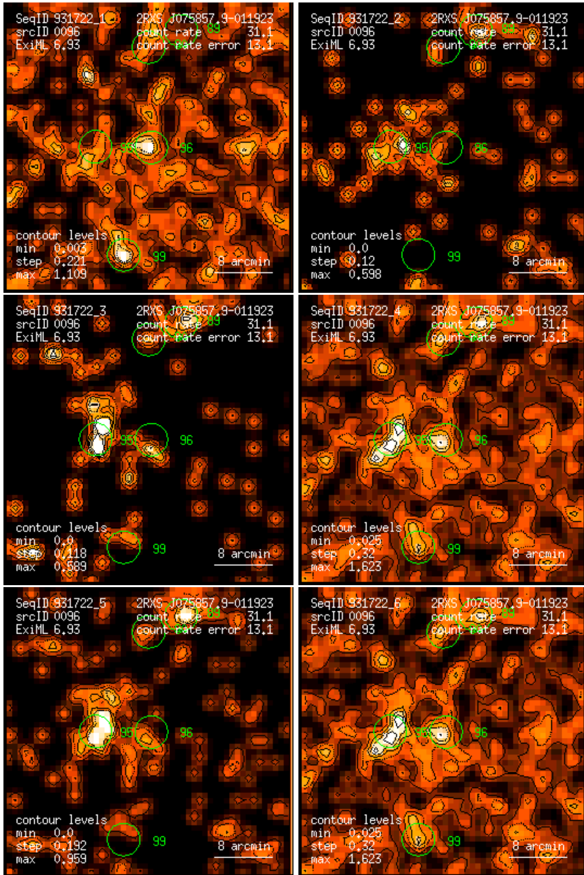
Figure 96: RASS 931722: detection 0096: band rate images, Gaussian filter: (1) PSPC channels 11 – 41, (2) 52 – 90, (3) 91 – 201, (4) 11 – 235, (5) 52 – 201, (6) 11 – 201. Broad band rates in counts/ks. Band rate contour levels in counts/ks/arcmin 2 .
