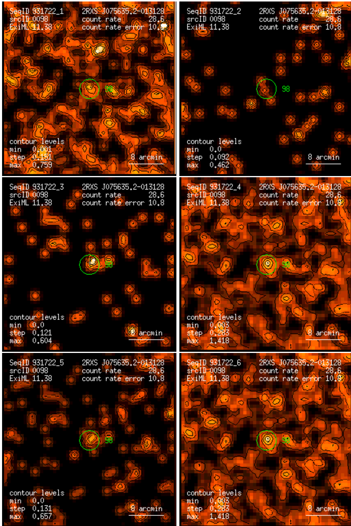
Figure 98: RASS 931722: detection 0098: band rate images, Gaussian filter: (1) PSPC channels 11 – 41, (2) 52 – 90, (3) 91 – 201, (4) 11 – 235, (5) 52 – 201, (6) 11 – 201. Broad band rates in counts/ks. Band rate contour levels in counts/ks/arcmin 2 .
