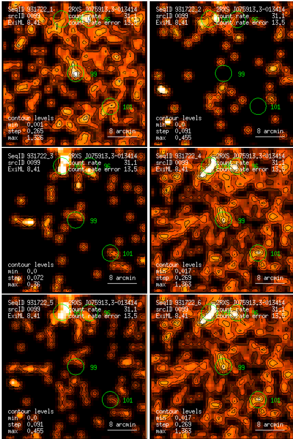
Figure 99: RASS 931722: detection 0099: band rate images, Gaussian filter: (1) PSPC channels 11 – 41, (2) 52 – 90, (3) 91 – 201, (4) 11 – 235, (5) 52 – 201, (6) 11 – 201. Broad band rates in counts/ks. Band rate contour levels in counts/ks/arcmin 2 .
