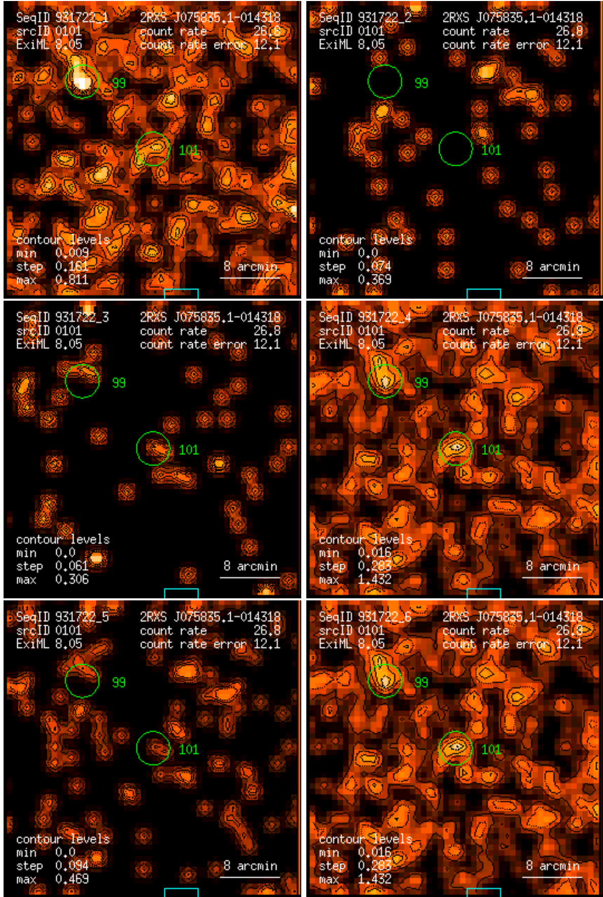
Figure 101: RASS 931722: detection 0101: band rate images, Gaussian filter: (1) PSPC channels 11 – 41, (2) 52 – 90, (3) 91 – 201, (4) 11 – 235, (5) 52 – 201, (6) 11 – 201. Broad band rates in counts/ks. Band rate contour levels in counts/ks/arcmin 2 .
