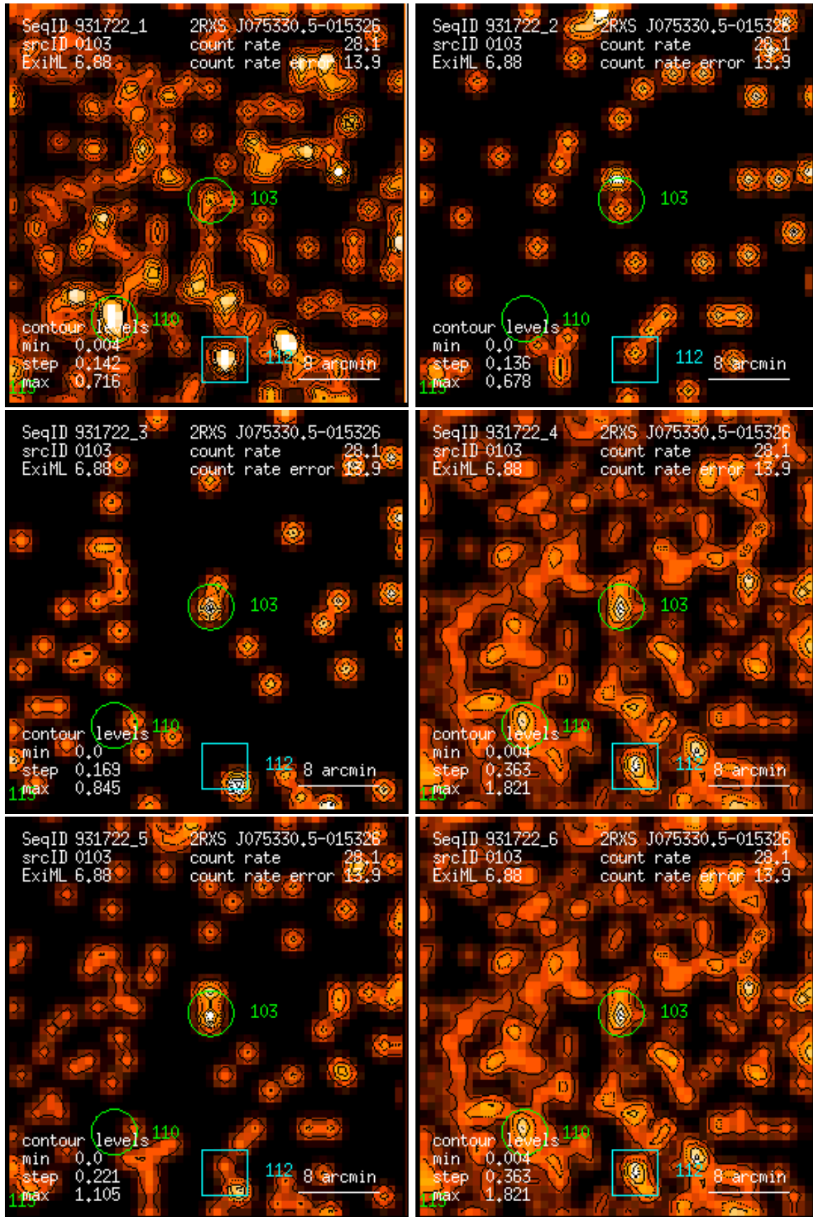
Figure 103: RASS 931722: detection 0103: band rate images, Gaussian filter: (1) PSPC channels 11 – 41, (2) 52 – 90, (3) 91 – 201, (4) 11 – 235, (5) 52 – 201, (6) 11 – 201. Broad band rates in counts/ks. Band rate contour levels in counts/ks/arcmin 2 .
