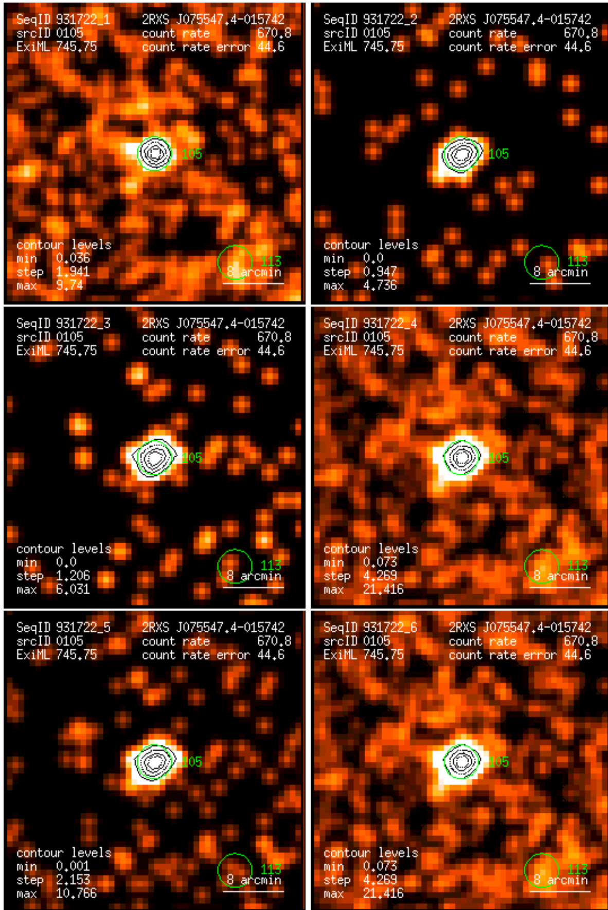
Figure 105: RASS 931722: detection 0105: band rate images, Gaussian filter: (1) PSPC channels 11 – 41, (2) 52 – 90, (3) 91 – 201, (4) 11 – 235, (5) 52 – 201, (6) 11 – 201. Broad band rates in counts/ks. Band rate contour levels in counts/ks/arcmin 2 .
