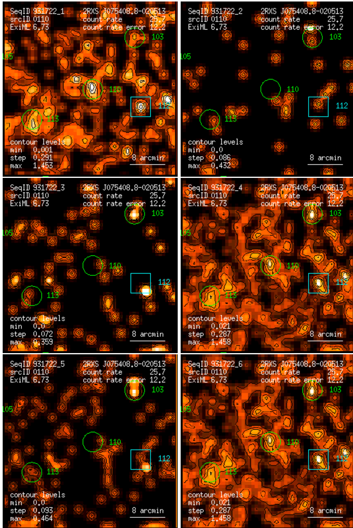
Figure 110: RASS 931722: detection 0110: band rate images, Gaussian filter: (1) PSPC channels 11 – 41, (2) 52 – 90, (3) 91 – 201, (4) 11 – 235, (5) 52 – 201, (6) 11 – 201. Broad band rates in counts/ks. Band rate contour levels in counts/ks/arcmin 2 .
