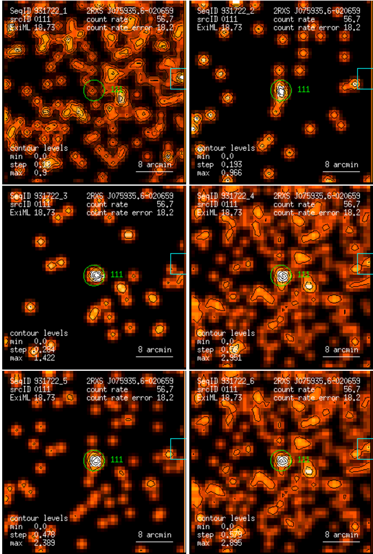
Figure 111: RASS 931722: detection 0111: band rate images, Gaussian filter: (1) PSPC channels 11 – 41, (2) 52 – 90, (3) 91 – 201, (4) 11 – 235, (5) 52 – 201, (6) 11 – 201. Broad band rates in counts/ks. Band rate contour levels in counts/ks/arcmin 2 .
