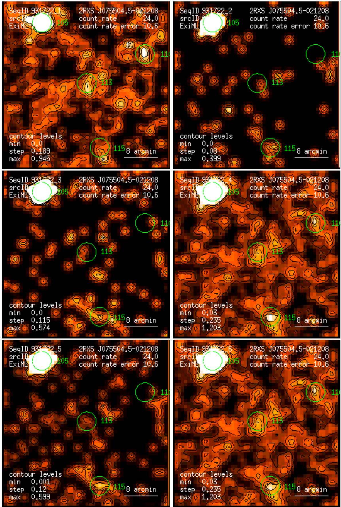
Figure 113: RASS 931722: detection 0113: band rate images, Gaussian filter: (1) PSPC channels 11 – 41, (2) 52 – 90, (3) 91 – 201, (4) 11 – 235, (5) 52 – 201, (6) 11 – 201. Broad band rates in counts/ks. Band rate contour levels in counts/ks/arcmin 2 .
