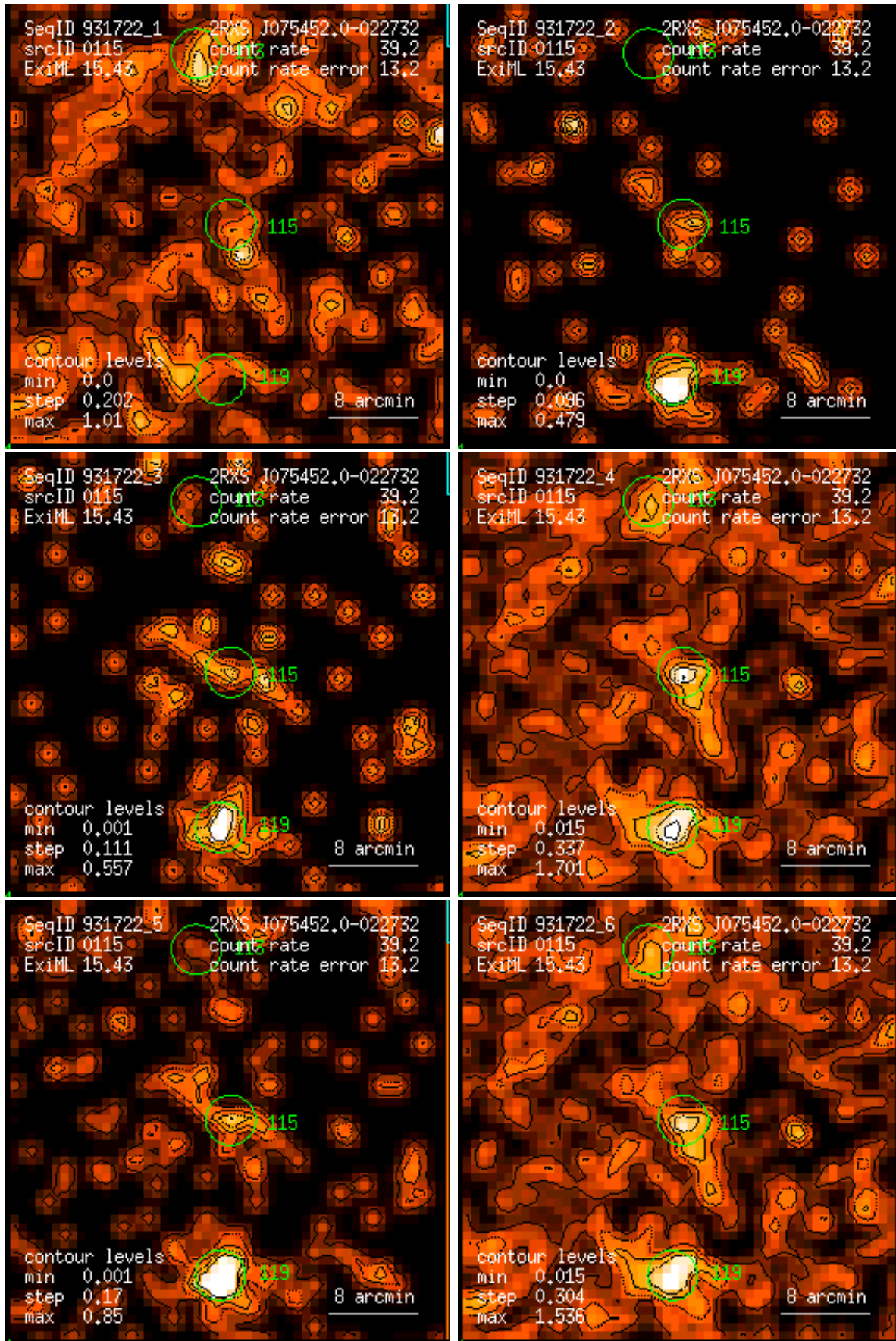
Figure 115: RASS 931722: detection 0115: band rate images, Gaussian filter: (1) PSPC channels 11 – 41, (2) 52 – 90, (3) 91 – 201, (4) 11 – 235, (5) 52 – 201, (6) 11 – 201. Broad band rates in counts/ks. Band rate contour levels in counts/ks/arcmin 2 .
