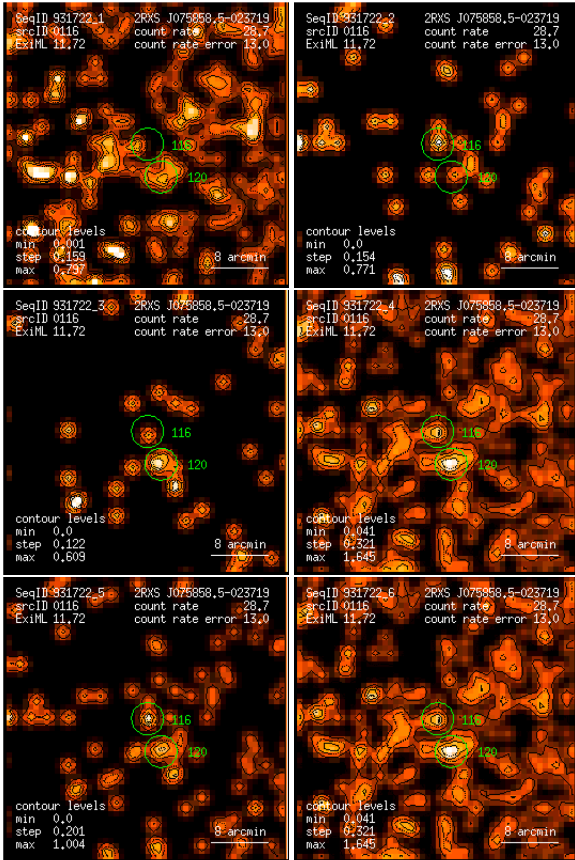
Figure 116: RASS 931722: detection 0116: band rate images, Gaussian filter: (1) PSPC channels 11 – 41, (2) 52 – 90, (3) 91 – 201, (4) 11 – 235, (5) 52 – 201, (6) 11 – 201. Broad band rates in counts/ks. Band rate contour levels in counts/ks/arcmin 2 .
