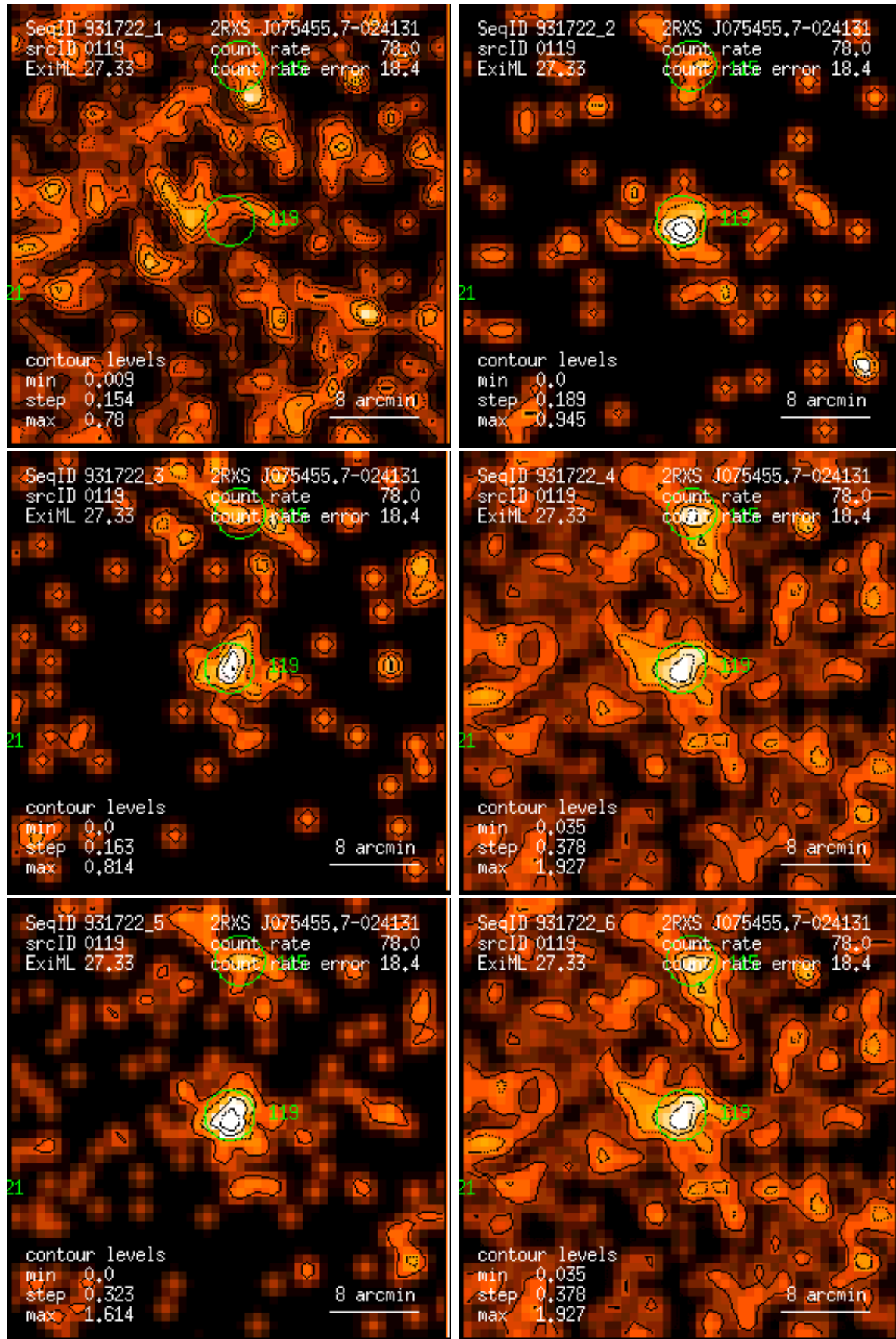
Figure 119: RASS 931722: detection 0119: band rate images, Gaussian filter: (1) PSPC channels 11 – 41, (2) 52 – 90, (3) 91 – 201, (4) 11 – 235, (5) 52 – 201, (6) 11 – 201. Broad band rates in counts/ks. Band rate contour levels in counts/ks/arcmin 2 .
