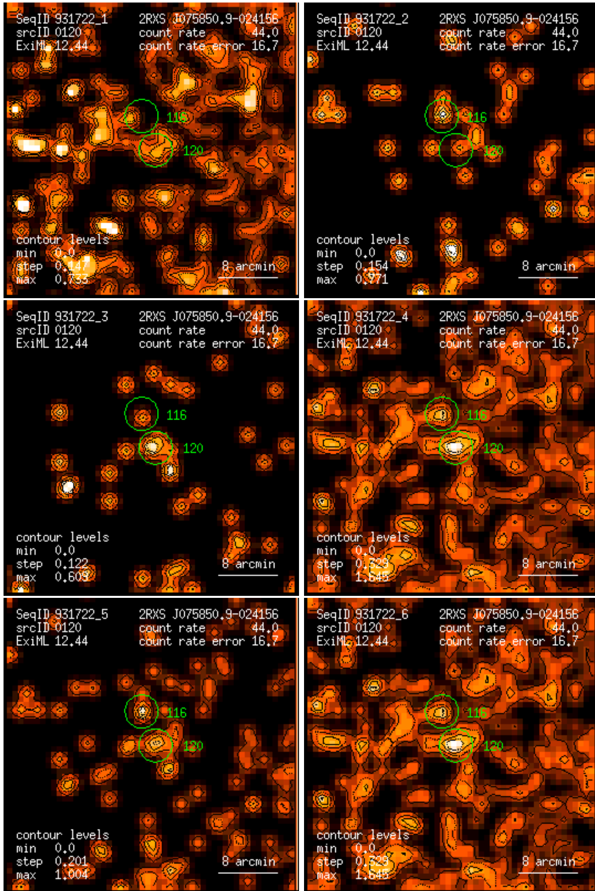
Figure 120: RASS 931722: detection 0120: band rate images, Gaussian filter: (1) PSPC channels 11 – 41, (2) 52 – 90, (3) 91 – 201, (4) 11 – 235, (5) 52 – 201, (6) 11 – 201. Broad band rates in counts/ks. Band rate contour levels in counts/ks/arcmin 2 .
