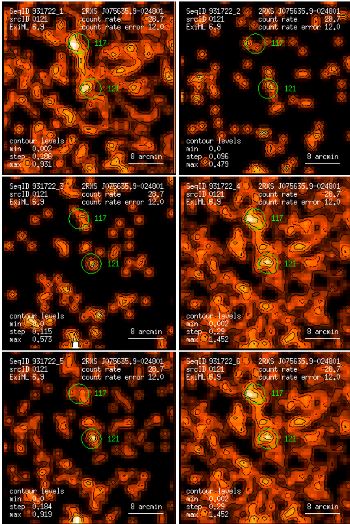
Figure 121: RASS 931722: detection 0121: band rate images, Gaussian filter: (1) PSPC channels 11 – 41, (2) 52 – 90, (3) 91 – 201, (4) 11 – 235, (5) 52 – 201, (6) 11 – 201. Broad band rates in counts/ks. Band rate contour levels in counts/ks/arcmin 2 .
