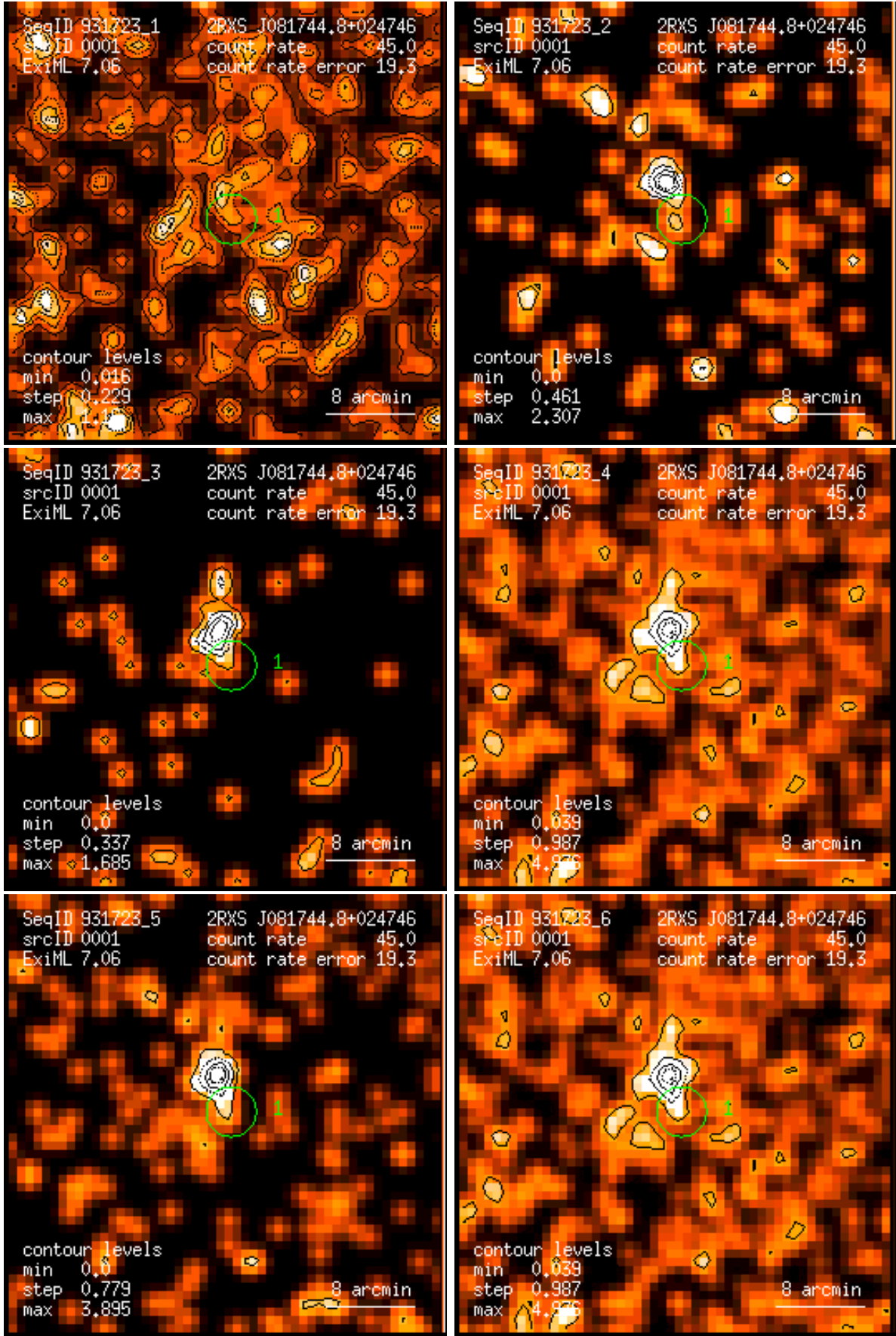
Figure 1: RASS 931723: detection 0001: band rate images, Gaussian filter: (1) PSPC channels 11 – 41, (2) 52 – 90, (3) 91 – 201, (4) 11 – 235, (5) 52 – 201, (6) 11 – 201. Broad band rates in counts/ks. Band rate contour levels in counts/ks/arcmin 2 .
