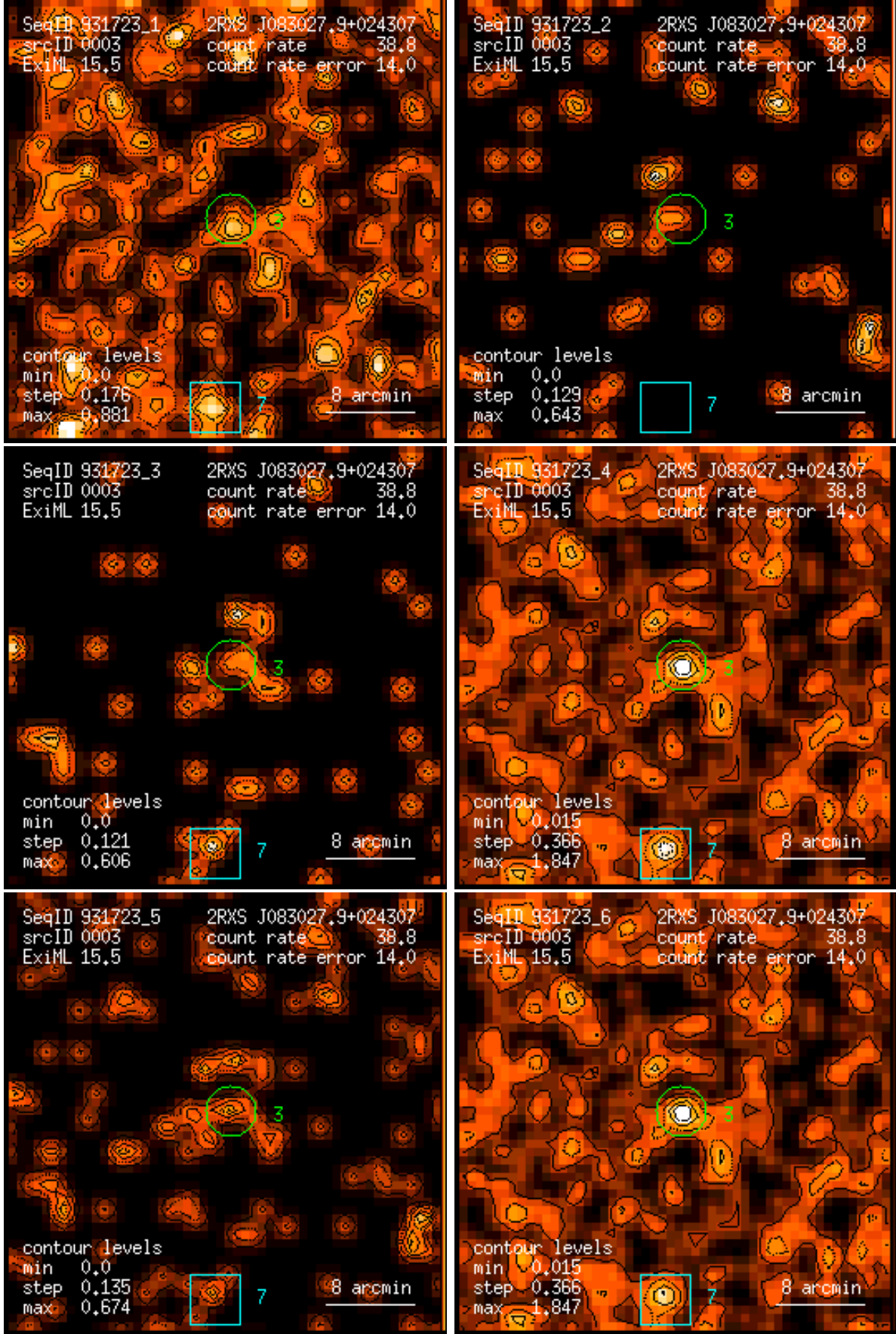
Figure 3: RASS 931723: detection 0003: band rate images, Gaussian filter: (1) PSPC channels 11 – 41, (2) 52 – 90, (3) 91 – 201, (4) 11 – 235, (5) 52 – 201, (6) 11 – 201. Broad band rates in counts/ks. Band rate contour levels in counts/ks/arcmin 2 .
