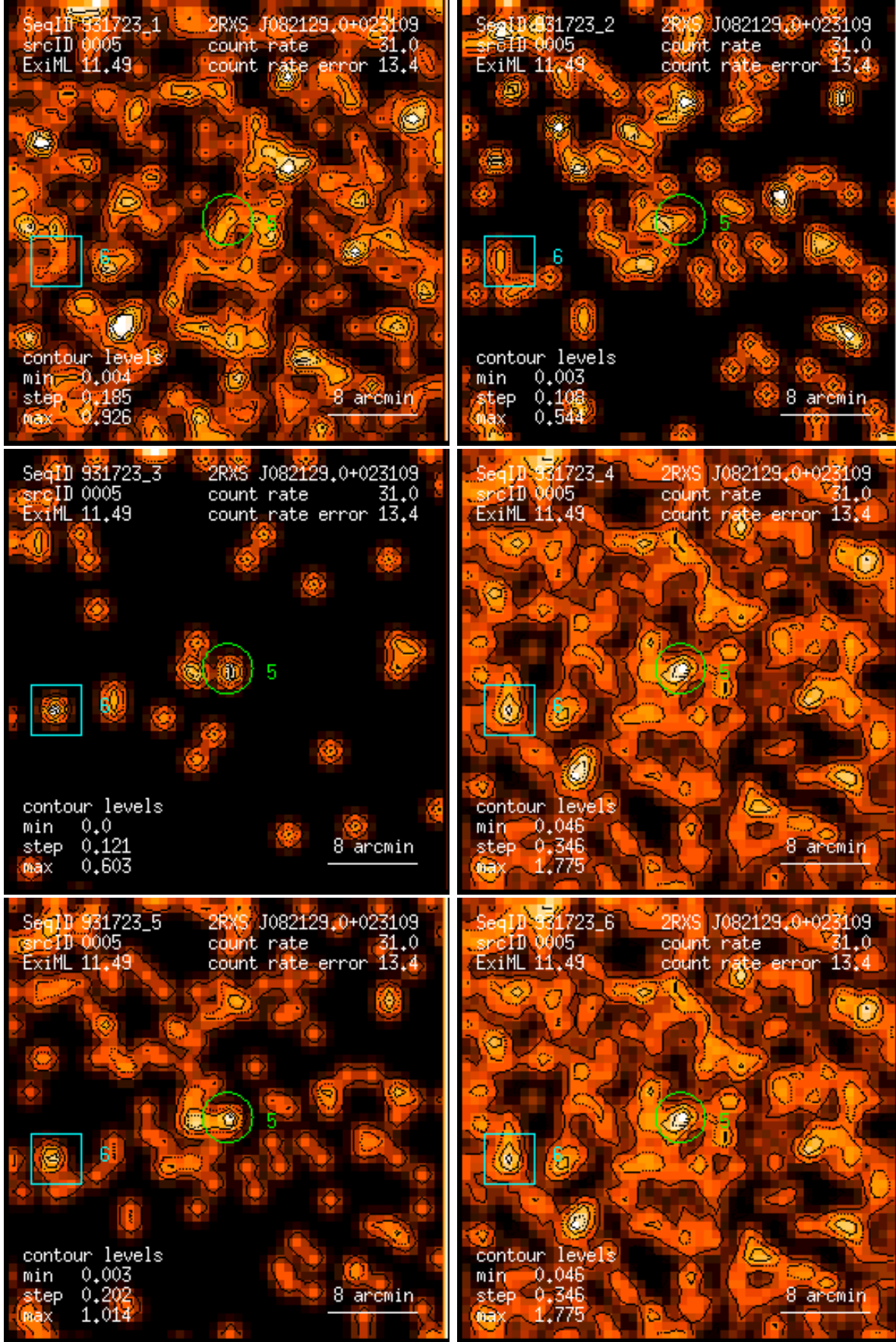
Figure 5: RASS 931723: detection 0005: band rate images, Gaussian filter: (1) PSPC channels 11 – 41, (2) 52 – 90, (3) 91 – 201, (4) 11 – 235, (5) 52 – 201, (6) 11 – 201. Broad band rates in counts/ks. Band rate contour levels in counts/ks/arcmin 2 .
