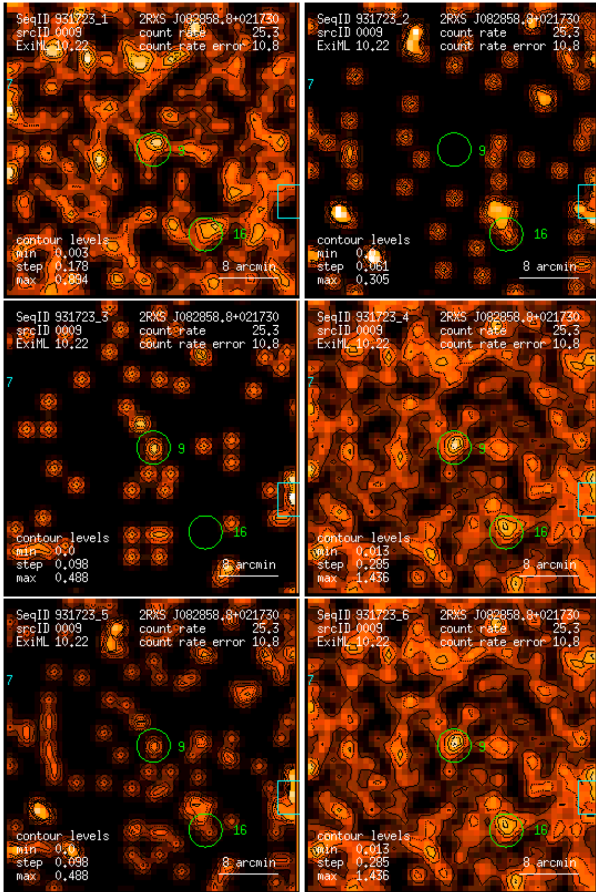
Figure 9: RASS 931723: detection 0009: band rate images, Gaussian filter: (1) PSPC channels 11 – 41, (2) 52 – 90, (3) 91 – 201, (4) 11 – 235, (5) 52 – 201, (6) 11 – 201. Broad band rates in counts/ks. Band rate contour levels in counts/ks/arcmin 2 .
