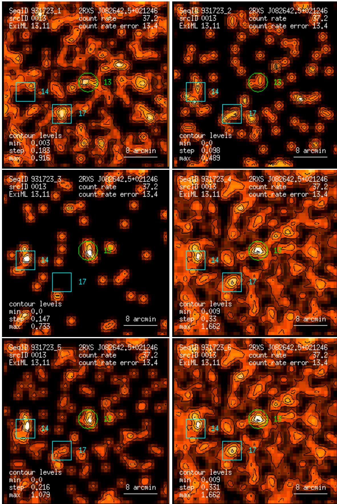
Figure 13: RASS 931723: detection 0013: band rate images, Gaussian filter: (1) PSPC channels 11 – 41, (2) 52 – 90, (3) 91 – 201, (4) 11 – 235, (5) 52 – 201, (6) 11 – 201. Broad band rates in counts/ks. Band rate contour levels in counts/ks/arcmin 2 .
