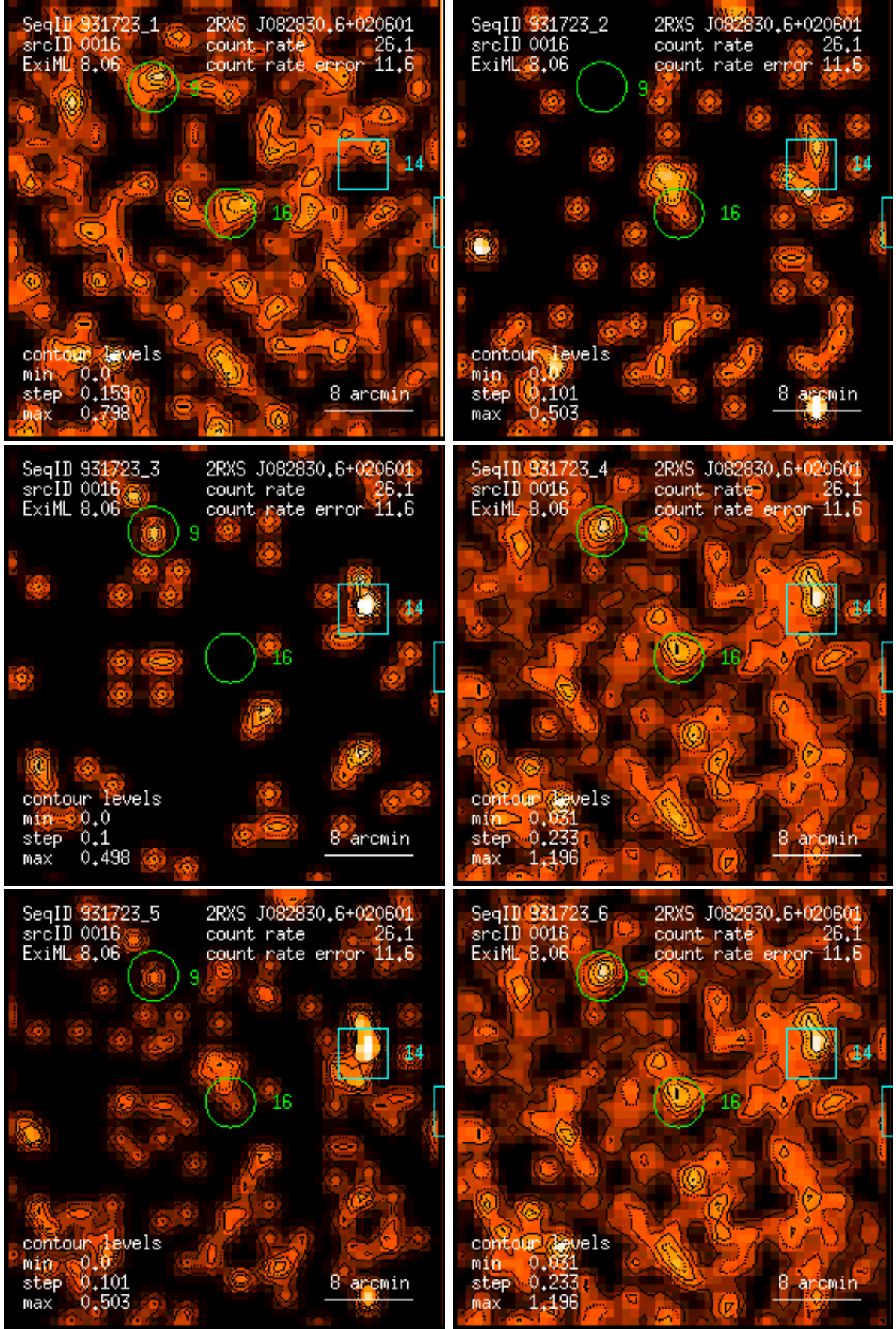
Figure 16: RASS 931723: detection 0016: band rate images, Gaussian filter: (1) PSPC channels 11 – 41, (2) 52 – 90, (3) 91 – 201, (4) 11 – 235, (5) 52 – 201, (6) 11 – 201. Broad band rates in counts/ks. Band rate contour levels in counts/ks/arcmin 2 .
