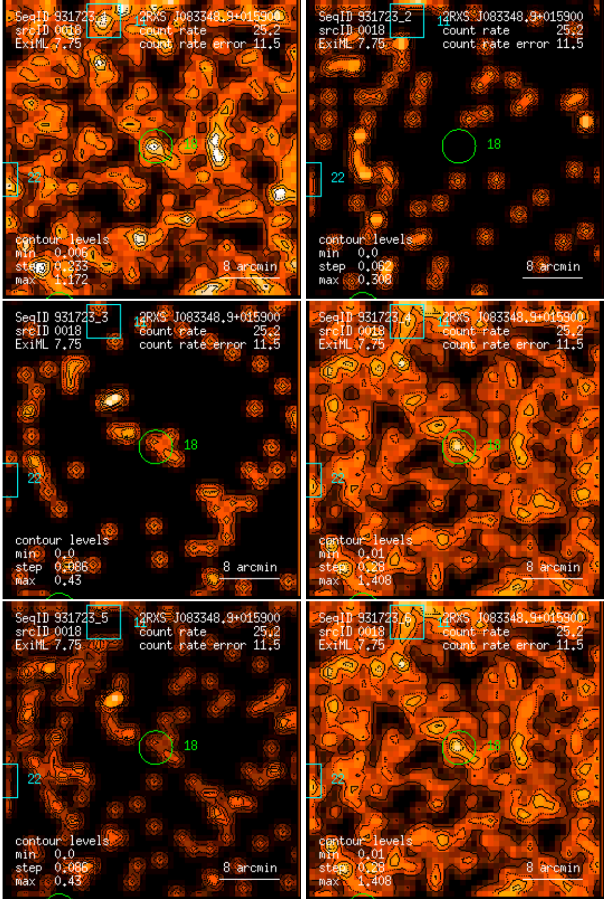
Figure 18: RASS 931723: detection 0018: band rate images, Gaussian filter: (1) PSPC channels 11 – 41, (2) 52 – 90, (3) 91 – 201, (4) 11 – 235, (5) 52 – 201, (6) 11 – 201. Broad band rates in counts/ks. Band rate contour levels in counts/ks/arcmin 2 .
