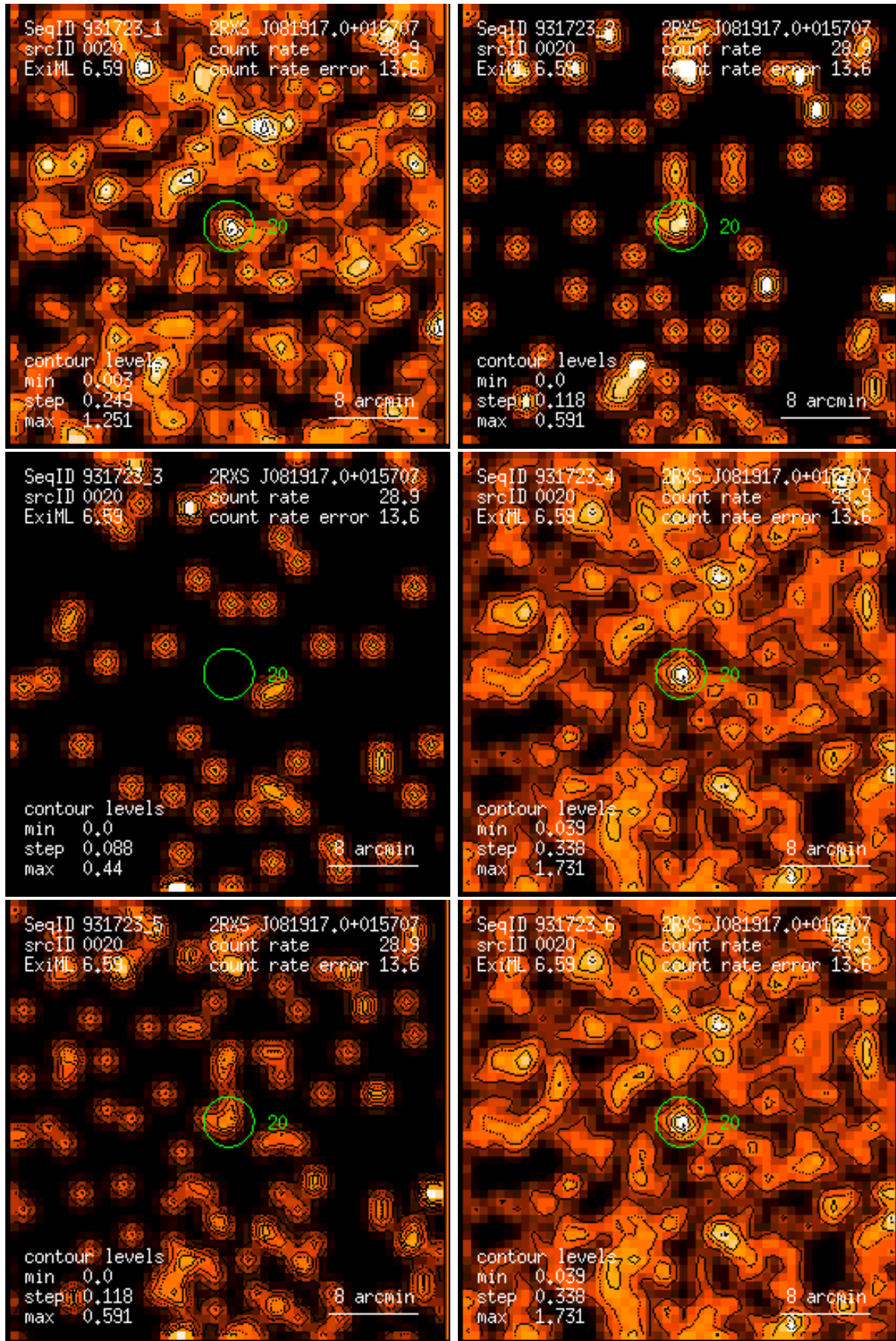
Figure 20: RASS 931723: detection 0020: band rate images, Gaussian filter: (1) PSPC channels 11 – 41, (2) 52 – 90, (3) 91 – 201, (4) 11 – 235, (5) 52 – 201, (6) 11 – 201. Broad band rates in counts/ks. Band rate contour levels in counts/ks/arcmin 2 .
