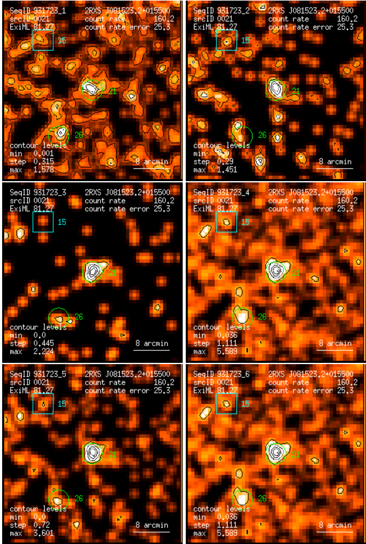
Figure 21: RASS 931723: detection 0021: band rate images, Gaussian filter: (1) PSPC channels 11 – 41, (2) 52 – 90, (3) 91 – 201, (4) 11 – 235, (5) 52 – 201, (6) 11 – 201. Broad band rates in counts/ks. Band rate contour levels in counts/ks/arcmin 2 .
