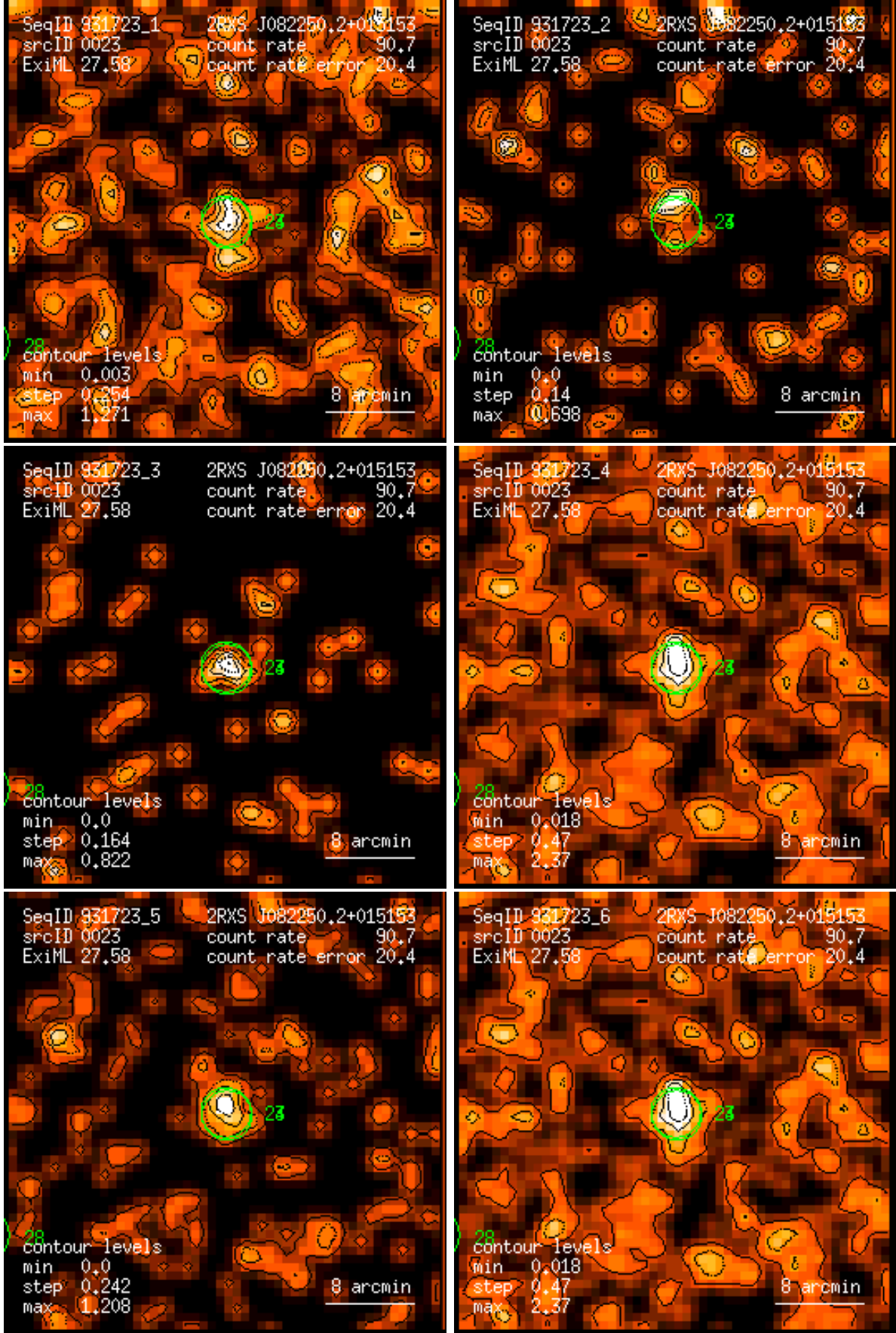
Figure 23: RASS 931723: detection 0023: band rate images, Gaussian filter: (1) PSPC channels 11 – 41, (2) 52 – 90, (3) 91 – 201, (4) 11 – 235, (5) 52 – 201, (6) 11 – 201. Broad band rates in counts/ks. Band rate contour levels in counts/ks/arcmin 2 .
