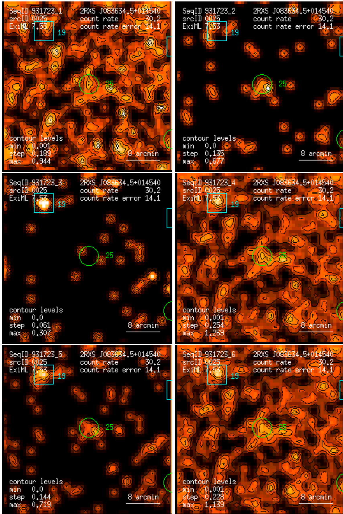
Figure 25: RASS 931723: detection 0025: band rate images, Gaussian filter: (1) PSPC channels 11 – 41, (2) 52 – 90, (3) 91 – 201, (4) 11 – 235, (5) 52 – 201, (6) 11 – 201. Broad band rates in counts/ks. Band rate contour levels in counts/ks/arcmin 2 .
