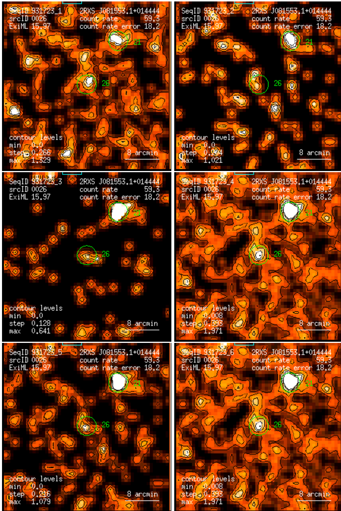
Figure 26: RASS 931723: detection 0026: band rate images, Gaussian filter: (1) PSPC channels 11 – 41, (2) 52 – 90, (3) 91 – 201, (4) 11 – 235, (5) 52 – 201, (6) 11 – 201. Broad band rates in counts/ks. Band rate contour levels in counts/ks/arcmin 2 .
