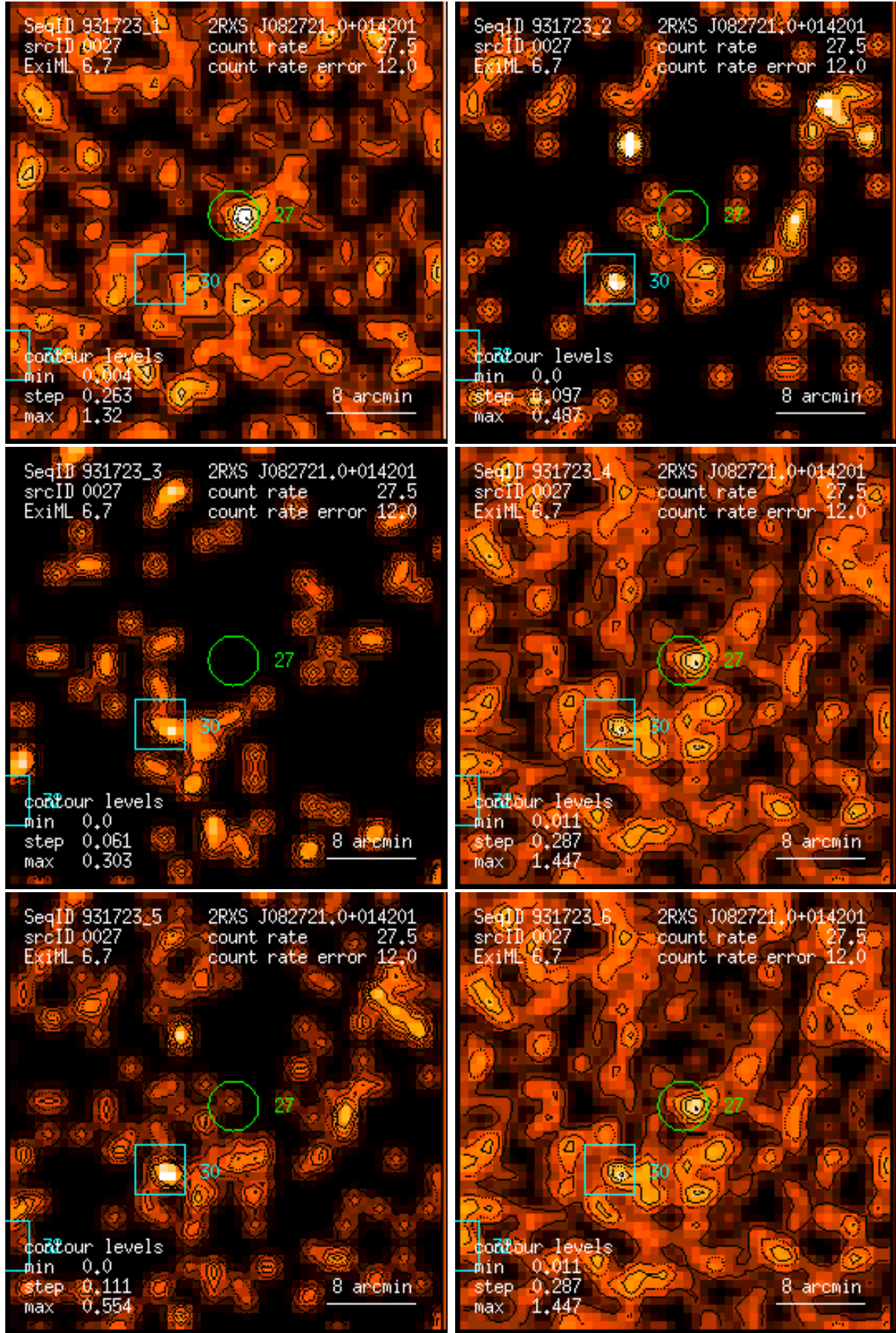
Figure 27: RASS 931723: detection 0027: band rate images, Gaussian filter: (1) PSPC channels 11 – 41, (2) 52 – 90, (3) 91 – 201, (4) 11 – 235, (5) 52 – 201, (6) 11 – 201. Broad band rates in counts/ks. Band rate contour levels in counts/ks/arcmin 2 .
