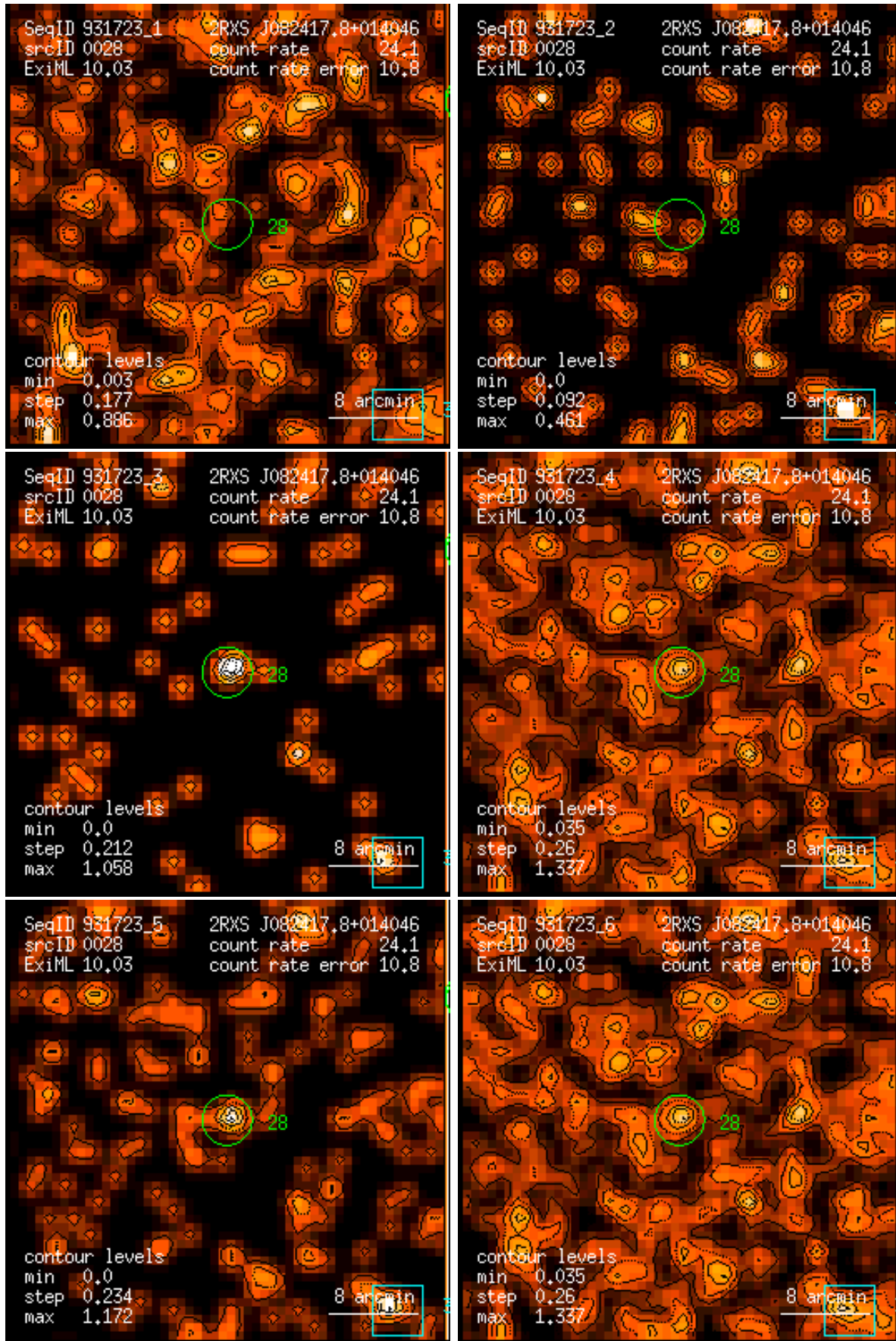
Figure 28: RASS 931723: detection 0028: band rate images, Gaussian filter: (1) PSPC channels 11 – 41, (2) 52 – 90, (3) 91 – 201, (4) 11 – 235, (5) 52 – 201, (6) 11 – 201. Broad band rates in counts/ks. Band rate contour levels in counts/ks/arcmin 2 .
