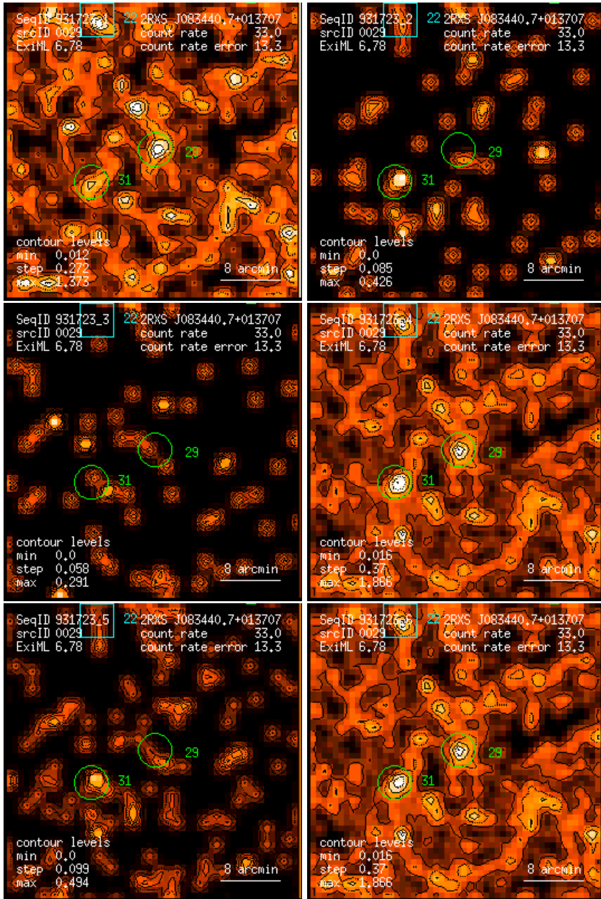
Figure 29: RASS 931723: detection 0029: band rate images, Gaussian filter: (1) PSPC channels 11 – 41, (2) 52 – 90, (3) 91 – 201, (4) 11 – 235, (5) 52 – 201, (6) 11 – 201. Broad band rates in counts/ks. Band rate contour levels in counts/ks/arcmin 2 .
