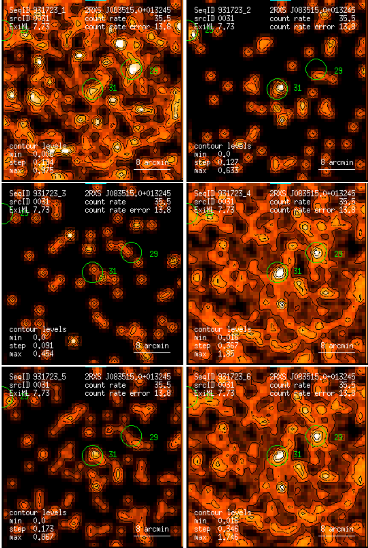
Figure 31: RASS 931723: detection 0031: band rate images, Gaussian filter: (1) PSPC channels 11 – 41, (2) 52 – 90, (3) 91 – 201, (4) 11 – 235, (5) 52 – 201, (6) 11 – 201. Broad band rates in counts/ks. Band rate contour levels in counts/ks/arcmin 2 .
