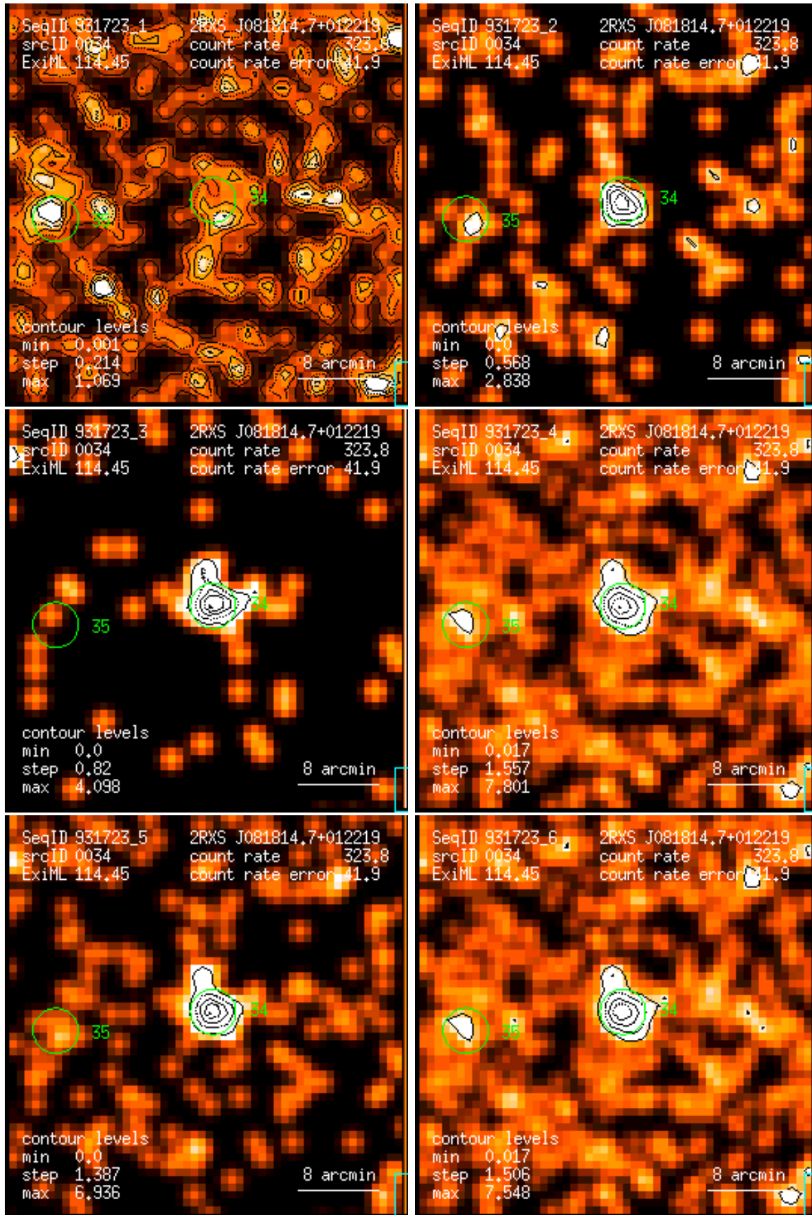
Figure 34: RASS 931723: detection 0034: band rate images, Gaussian filter: (1) PSPC channels 11 – 41, (2) 52 – 90, (3) 91 – 201, (4) 11 – 235, (5) 52 – 201, (6) 11 – 201. Broad band rates in counts/ks. Band rate contour levels in counts/ks/arcmin 2 .
