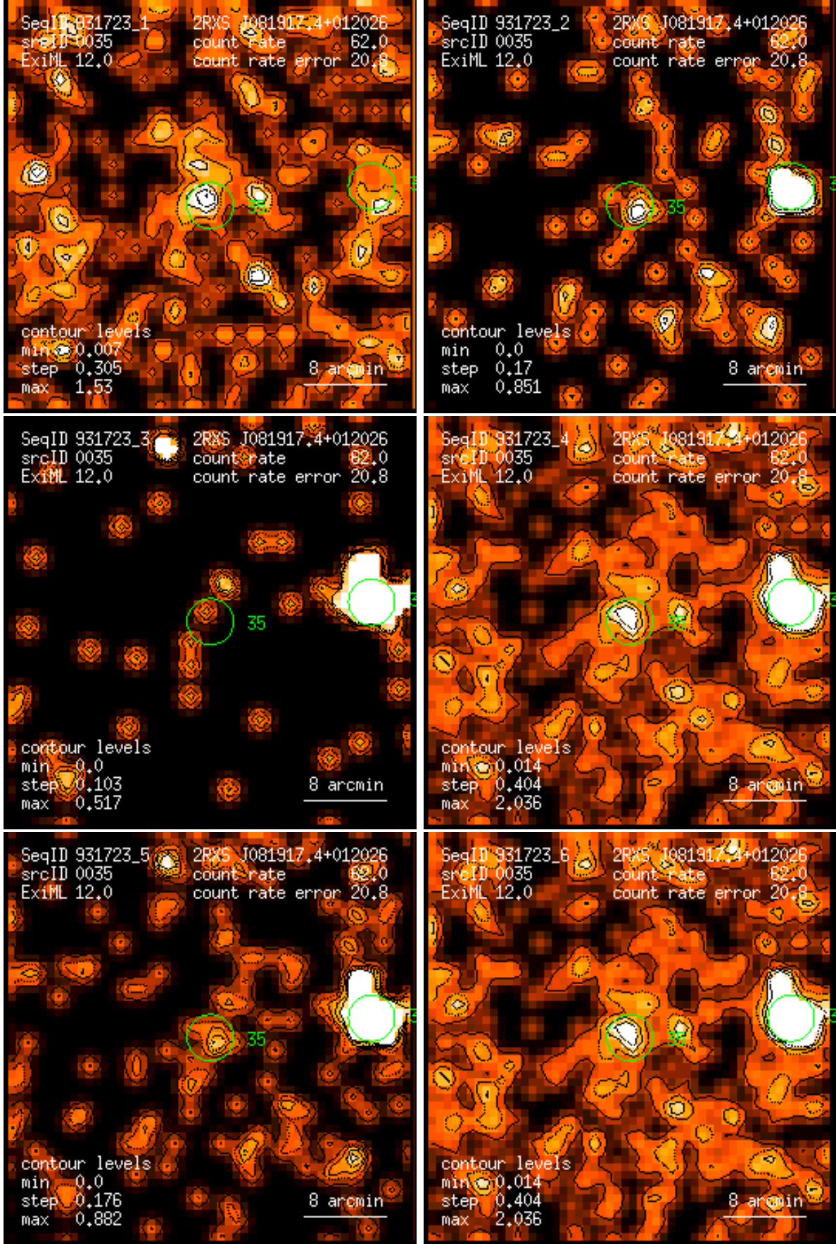
Figure 35: RASS 931723: detection 0035: band rate images, Gaussian filter: (1) PSPC channels 11 – 41, (2) 52 – 90, (3) 91 – 201, (4) 11 – 235, (5) 52 – 201, (6) 11 – 201. Broad band rates in counts/ks. Band rate contour levels in counts/ks/arcmin 2 .
