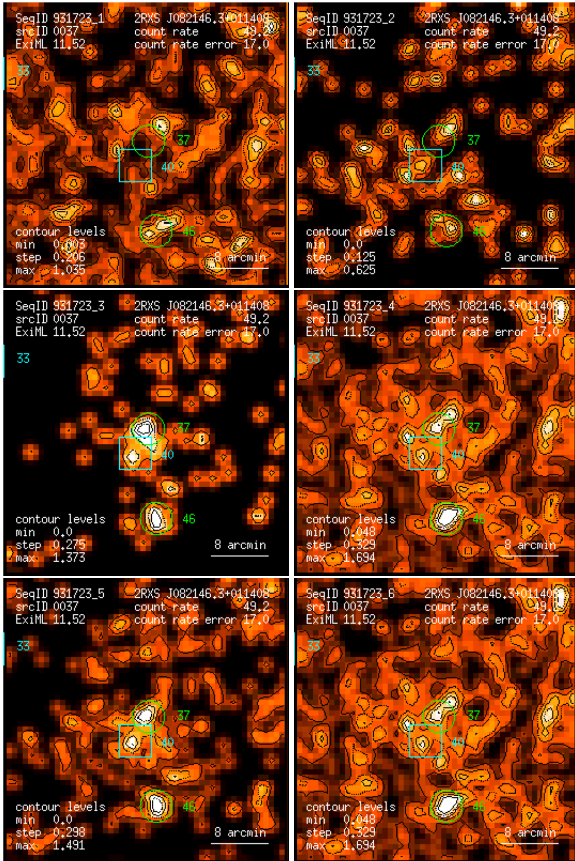
Figure 37: RASS 931723: detection 0037: band rate images, Gaussian filter: (1) PSPC channels 11 – 41, (2) 52 – 90, (3) 91 – 201, (4) 11 – 235, (5) 52 – 201, (6) 11 – 201. Broad band rates in counts/ks. Band rate contour levels in counts/ks/arcmin 2 .
