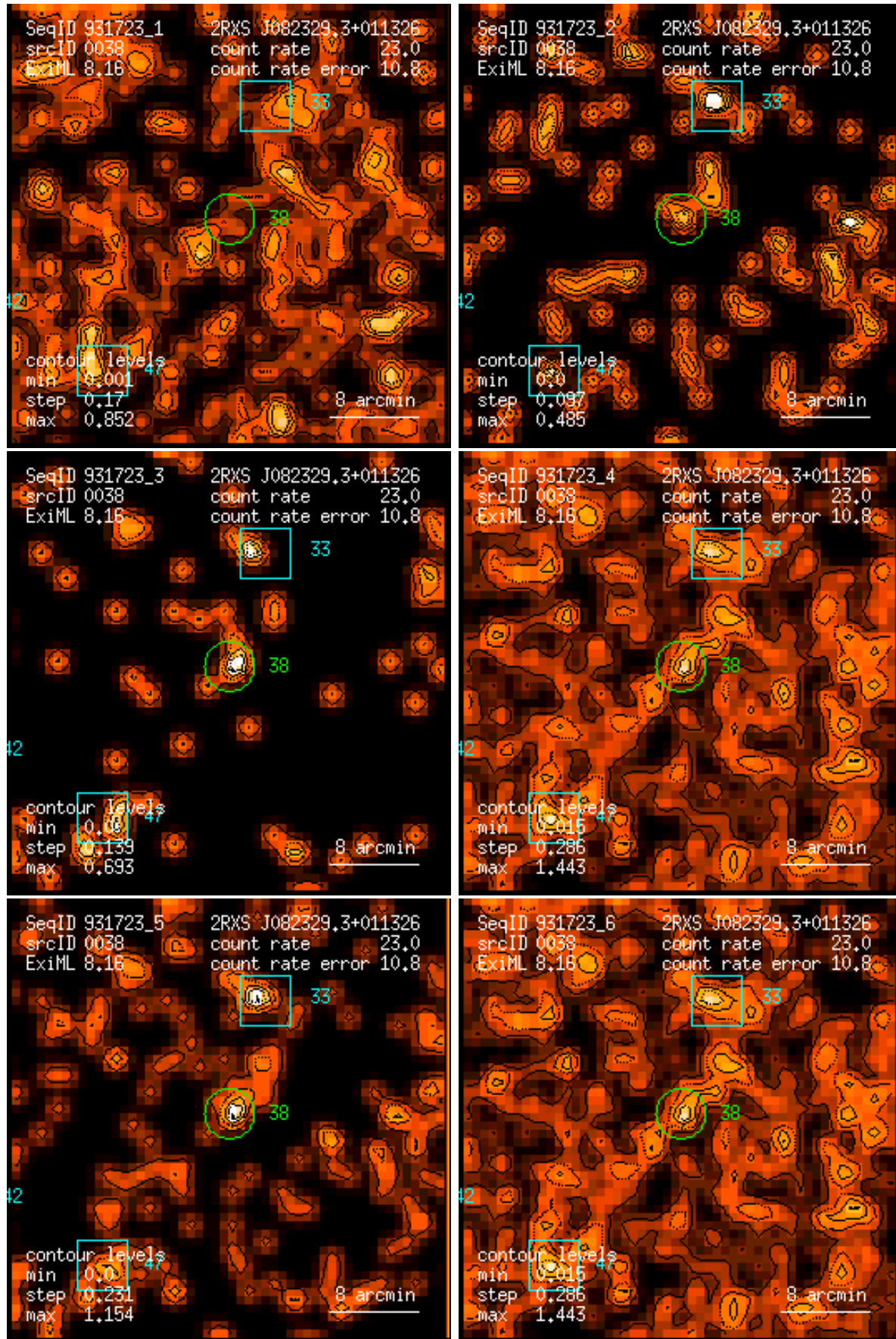
Figure 38: RASS 931723: detection 0038: band rate images, Gaussian filter: (1) PSPC channels 11 – 41, (2) 52 – 90, (3) 91 – 201, (4) 11 – 235, (5) 52 – 201, (6) 11 – 201. Broad band rates in counts/ks. Band rate contour levels in counts/ks/arcmin 2 .
