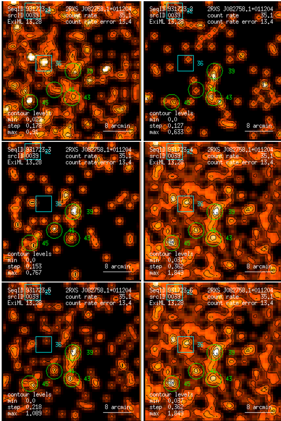
Figure 39: RASS 931723: detection 0039: band rate images, Gaussian filter: (1) PSPC channels 11 – 41, (2) 52 – 90, (3) 91 – 201, (4) 11 – 235, (5) 52 – 201, (6) 11 – 201. Broad band rates in counts/ks. Band rate contour levels in counts/ks/arcmin 2 .
