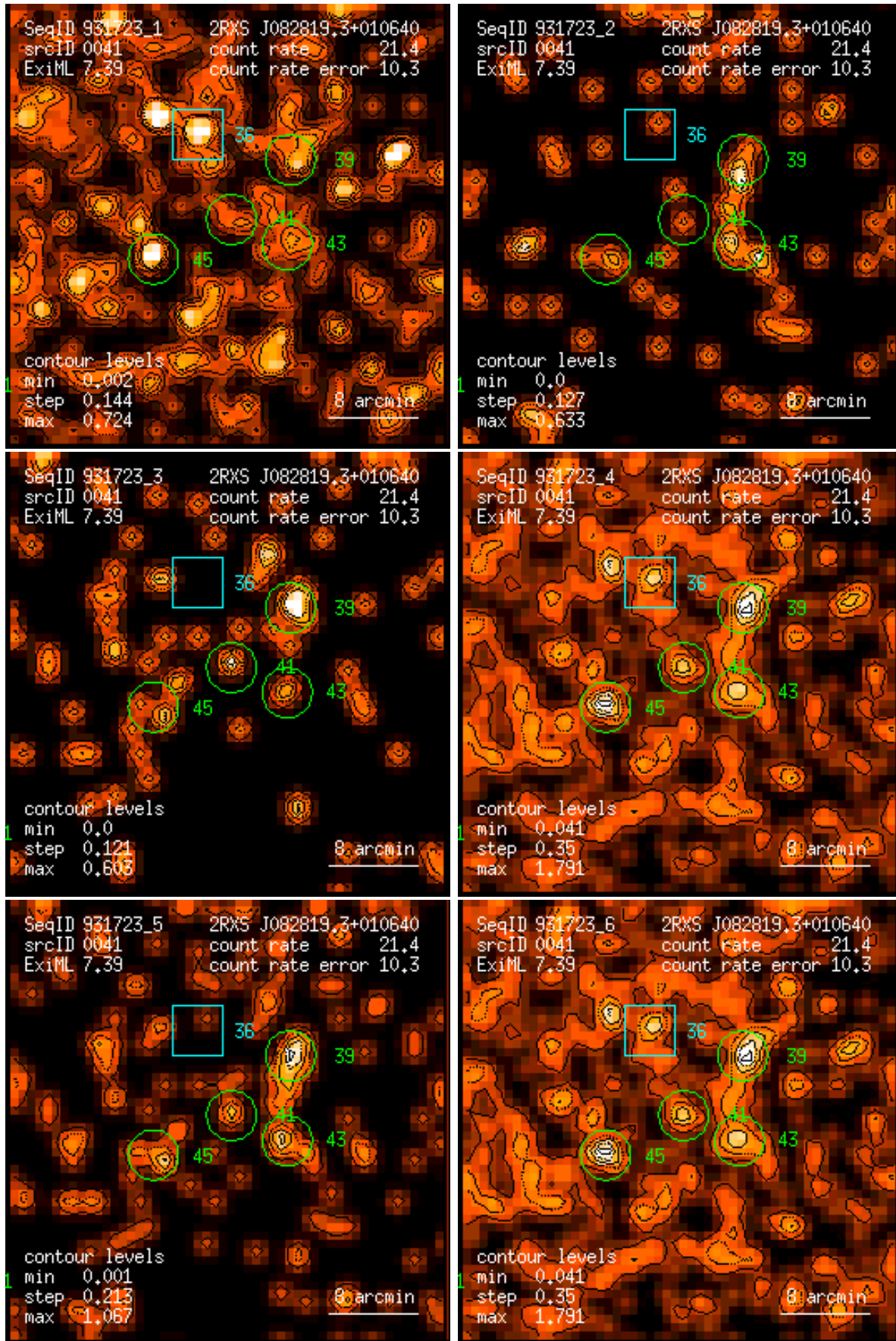
Figure 41: RASS 931723: detection 0041: band rate images, Gaussian filter: (1) PSPC channels 11 – 41, (2) 52 – 90, (3) 91 – 201, (4) 11 – 235, (5) 52 – 201, (6) 11 – 201. Broad band rates in counts/ks. Band rate contour levels in counts/ks/arcmin 2 .
