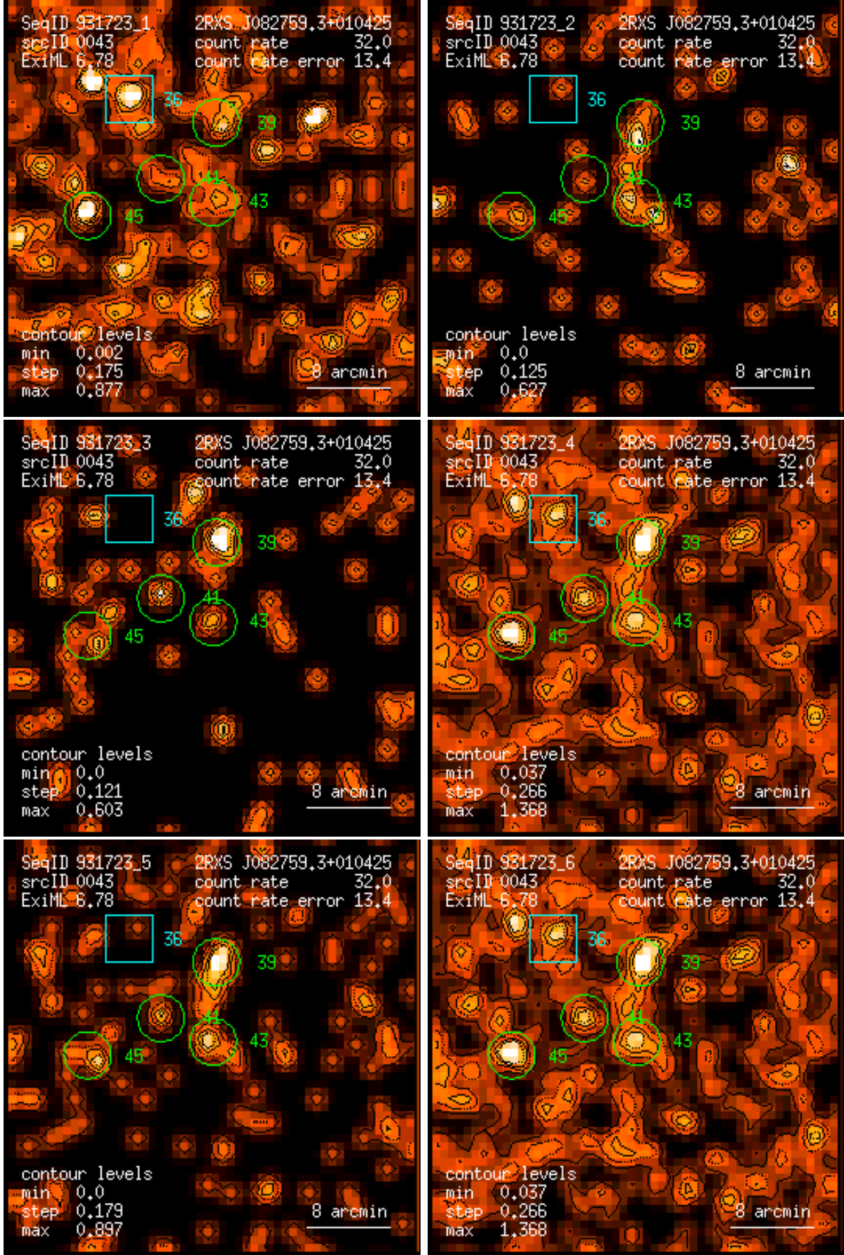
Figure 43: RASS 931723: detection 0043: band rate images, Gaussian filter: (1) PSPC channels 11 – 41, (2) 52 – 90, (3) 91 – 201, (4) 11 – 235, (5) 52 – 201, (6) 11 – 201. Broad band rates in counts/ks. Band rate contour levels in counts/ks/arcmin 2 .
